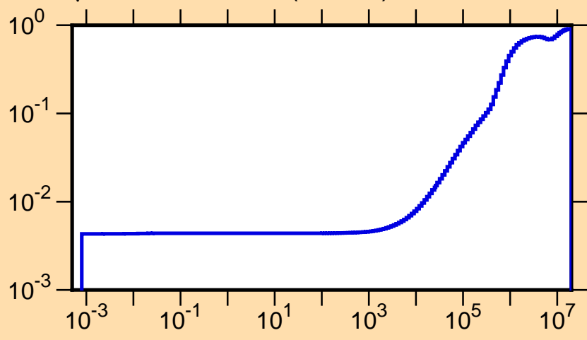
\mu vs. E for ^{156}\text{Tb}(\text{mt251})
