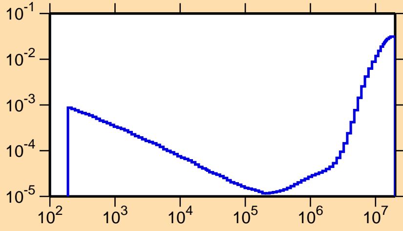
\sigma vs. E for ^{156}\text{Tb}(n,p)
