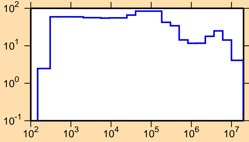
\Delta\sigma/\sigma vs. E for ^{156}\text{Tb}(n,el.)
