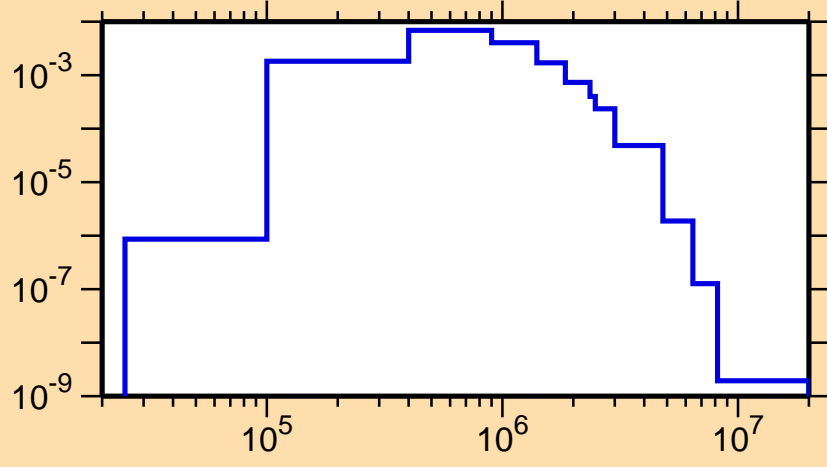
\sigma vs. E for ^{156}\text{Tb}(n,n_3)
