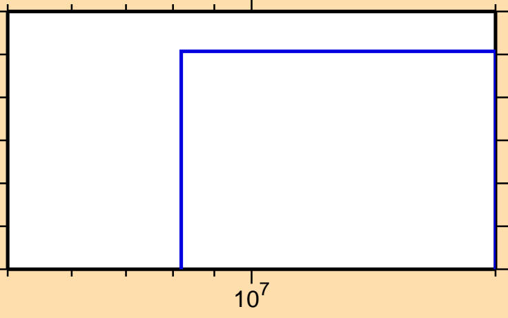
\sigma vs. E for ^{156}\text{Tb}(n,nt)
