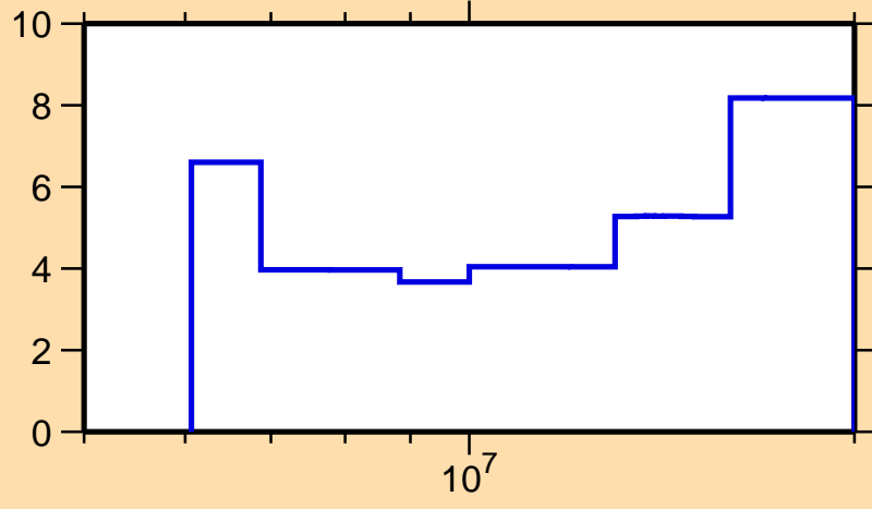
\Delta\sigma/\sigma vs. E for ^{156}\text{Tb}(n,\text{tot.})
