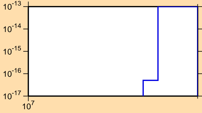
\sigma vs. E for ^{156}\text{Tb} (mt 34)
