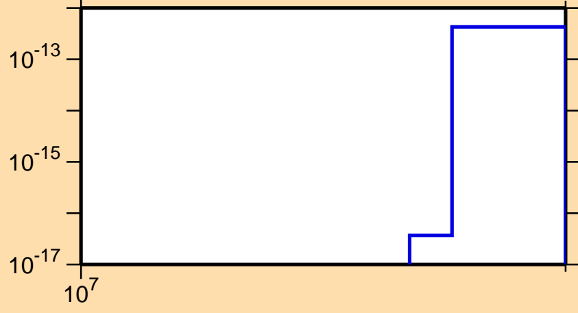
\sigma vs. E for ^{156}\text{Tb}(n,3n\alpha)
