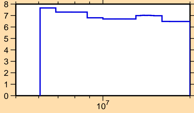
\Delta\sigma/\sigma vs. E for ^{156}\text{Tb}(n,\text{nonel.})
