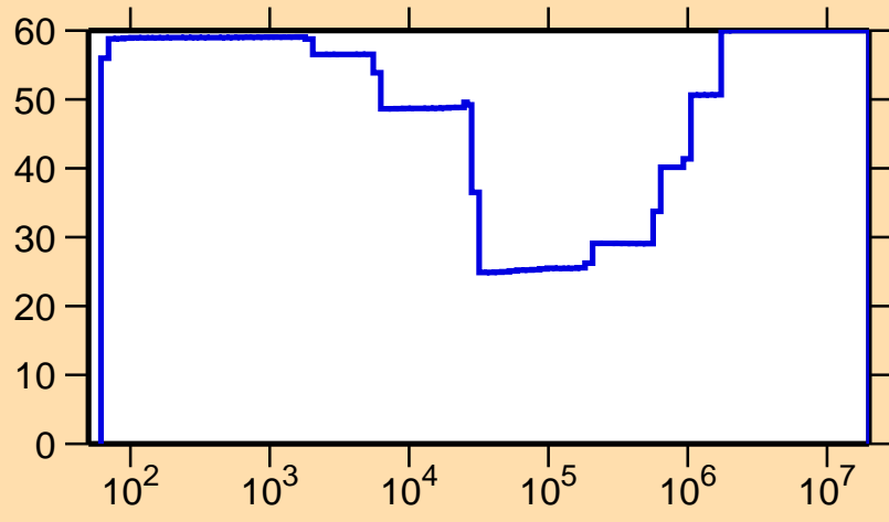
\Delta\sigma/\sigma vs. E for ^{156}\text{Tb}(n,\gamma)
