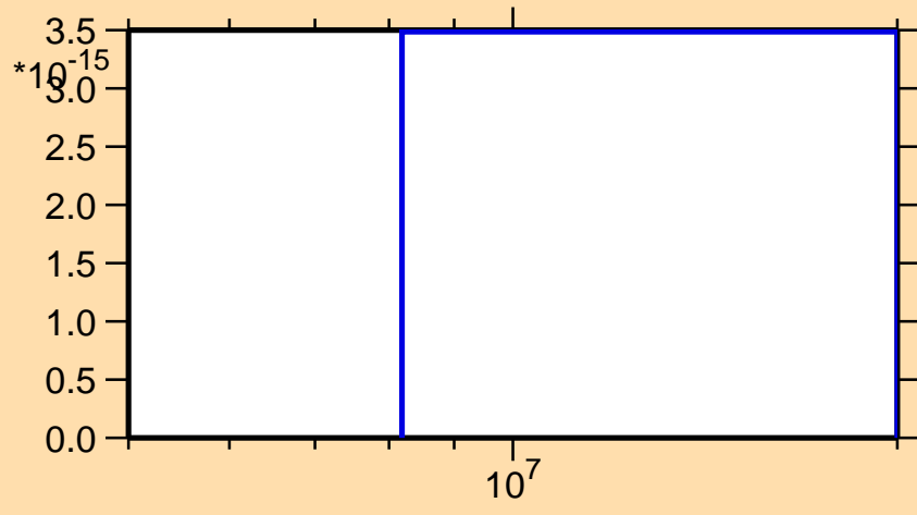
\sigma vs. E for ^{156}\text{Tb}(n,3n\alpha)
