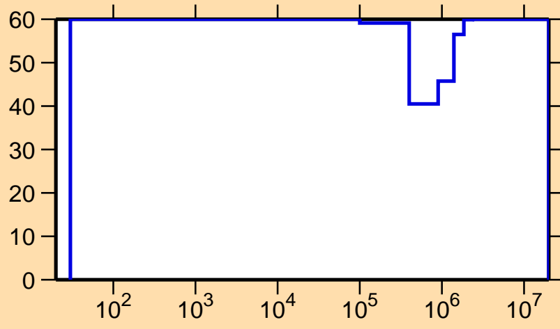
\Delta\sigma/\sigma vs. E for ^{156}\text{Tb}(n,n_1)
