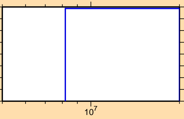
\sigma vs. E for ^{156}\text{Tb}(n,3n)
