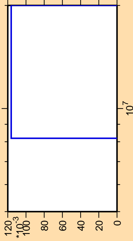
\Delta\sigma/\sigma vs. E for ^{156}\text{Tb}(\text{mt } 45)
