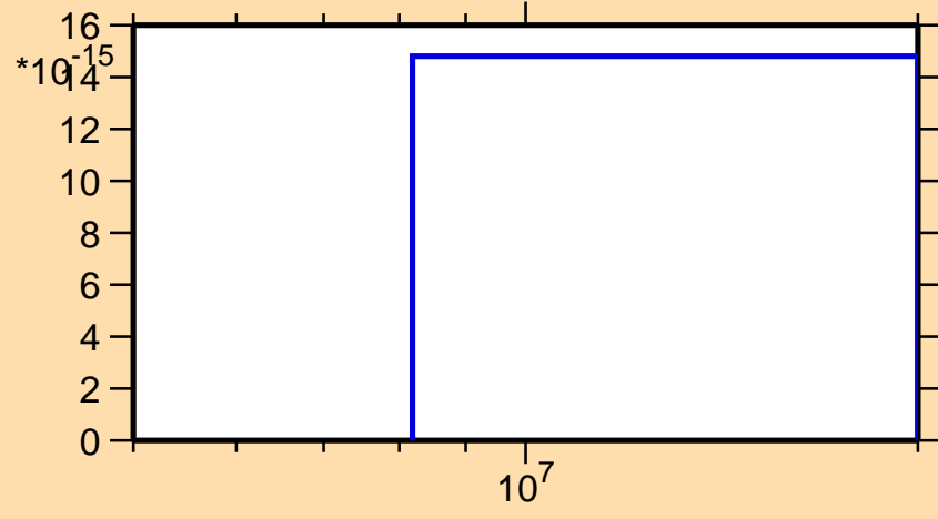
\sigma vs. E for ^{156}\text{Tb}(\text{mt } 45)
