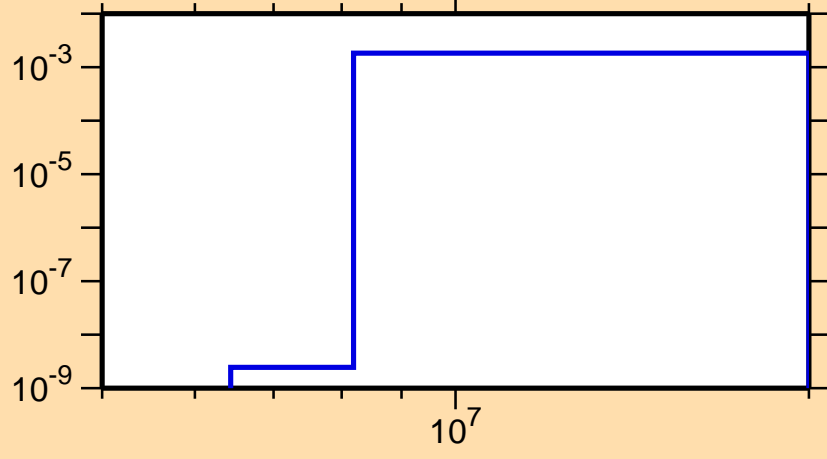
\sigma vs. E for ^{156}\text{Tb}(n,np)
