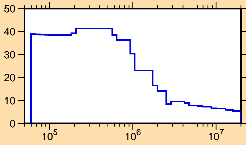
\Delta\sigma/\sigma vs. E for ^{157}\text{Tb}(n,\text{nonel.})
