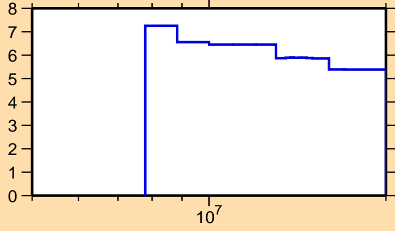
\Delta\sigma/\sigma vs. E for ^{157}\text{Tb}(n,\text{nonel.})
