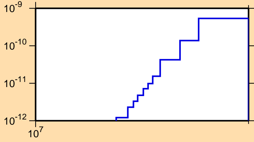
\sigma vs. E for ^{157}\text{Tb}(n,p\alpha)
