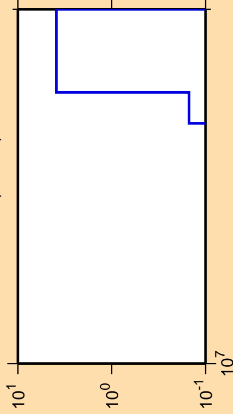
\Delta\sigma/\sigma vs. E for ^{157}\text{Tb} (mt 45)
