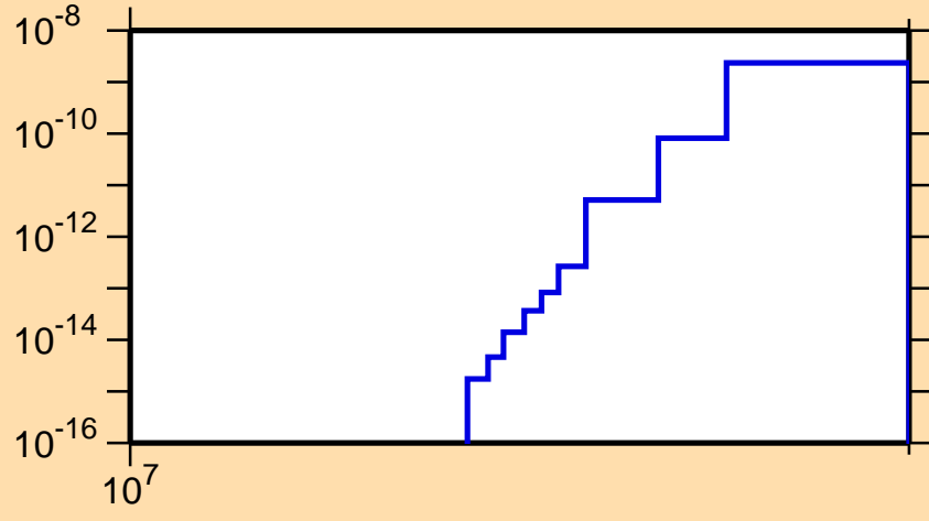
\sigma vs. E for ^{157}\text{Tb}(n,\text{He3})
