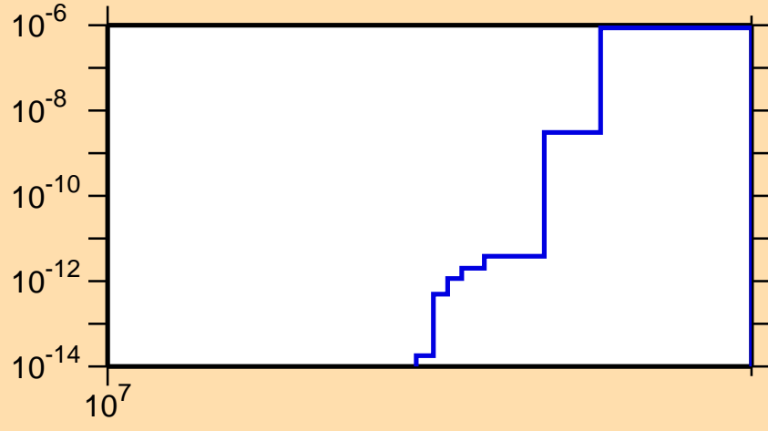
\sigma vs. E for ^{157}\text{Tb}(n,2np)
