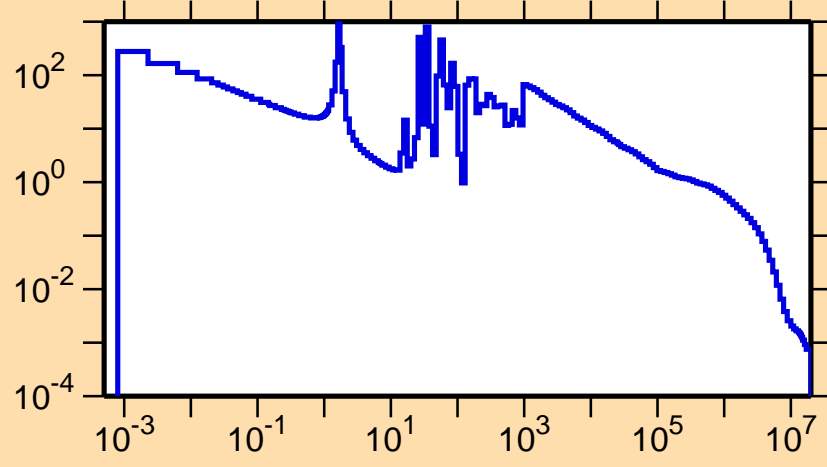
\sigma vs. E for ^{157}\text{Tb}(n,\gamma)
