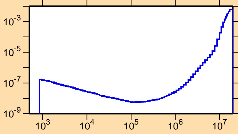
\sigma vs. E for ^{157}\text{Tb}(n,\alpha)
