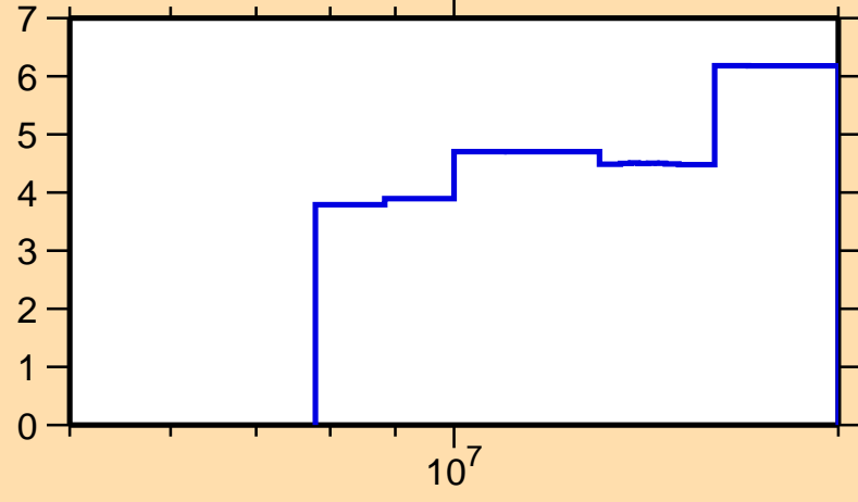
\Delta\sigma/\sigma vs. E for ^{157}\text{Tb}(n,\text{tot.})
