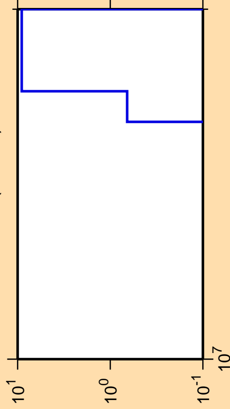
\Delta\sigma/\sigma vs. E for ^{157}\text{Tb}(\text{mt117})
