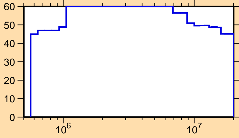
\Delta\sigma/\sigma vs. E for ^{157}\text{Tb}(n,n_1)
