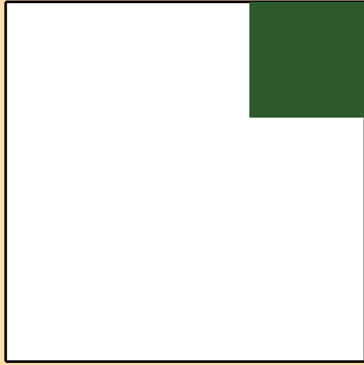
\sigma vs. E for ^{157}\text{Tb}(\text{mt117})
