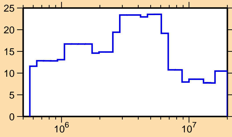
\Delta\sigma/\sigma vs. E for ^{157}\text{Tb}(n,\text{el.})
