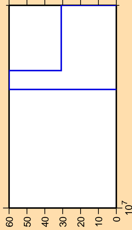
\Delta\sigma/\sigma vs. E for ^{157}\text{Tb}(n,3n)
