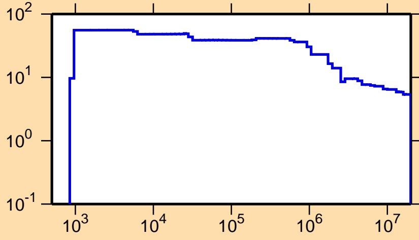
\Delta\sigma/\sigma vs. E for ^{157}\text{Tb}(n,\text{nonel.})
