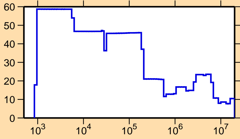
\Delta\sigma/\sigma vs. E for ^{157}\text{Tb}(n,\text{el.})
