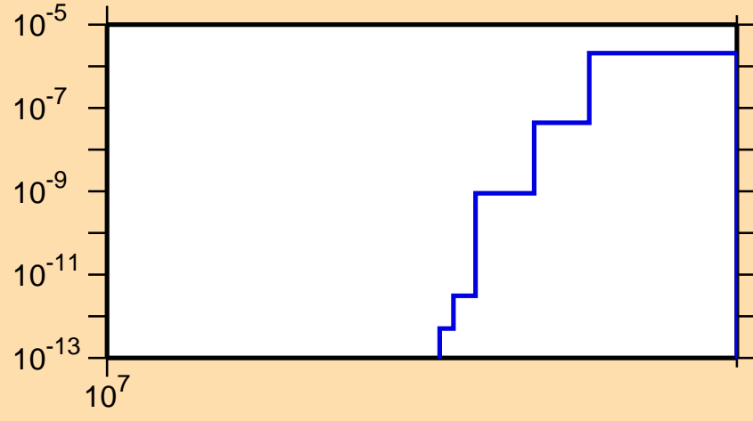
\sigma vs. E for ^{157}\text{Tb}(n,\text{nd})
