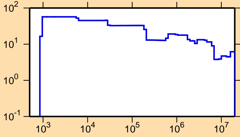
\Delta\sigma/\sigma vs. E for ^{157}\text{Tb}(n,\text{tot.})
