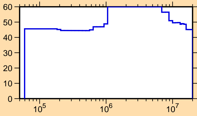
\Delta\sigma/\sigma vs. E for ^{157}\text{Tb}(n,n_1)
