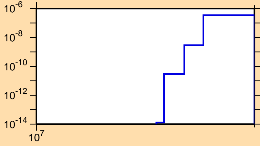
\sigma vs. E for ^{157}\text{Tb}(n,nt)
