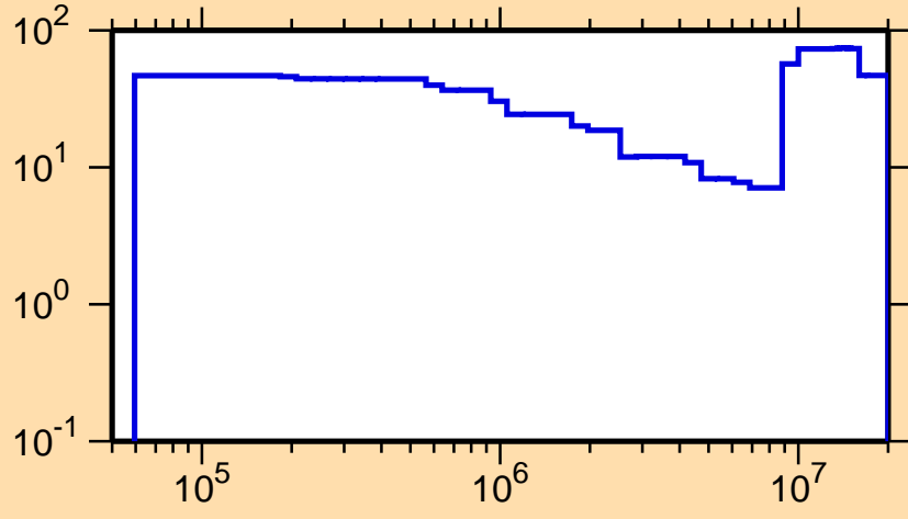
\Delta\sigma/\sigma vs. E for ^{157}\text{Tb}(n,\text{inel.})
