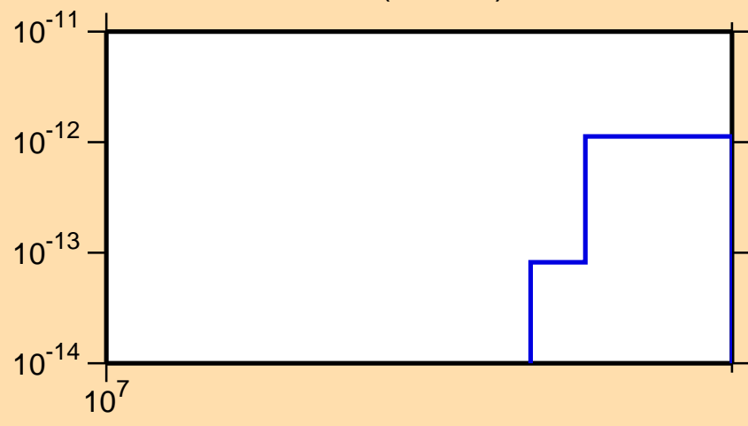
\sigma vs. E for ^{157}\text{Tb}(\text{mt117})
