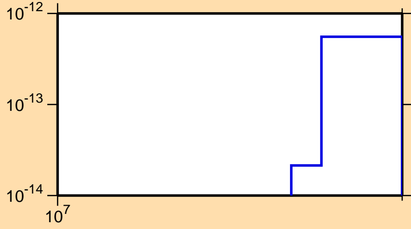
\sigma vs. E for ^{157}\text{Tb} (mt 45)
