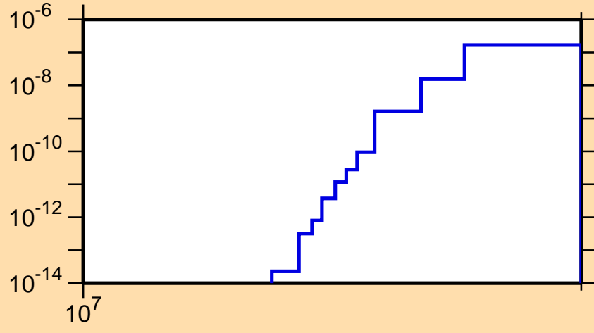
\sigma vs. E for ^{157}\text{Tb}(n,2n\alpha)
