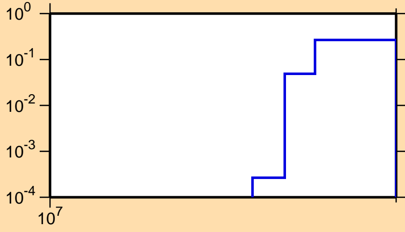
\sigma vs. E for ^{157}\text{Tb}(n,3n)
