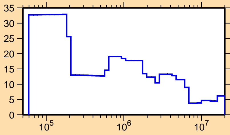
\Delta\sigma/\sigma vs. E for ^{157}\text{Tb}(n,\text{tot.})
