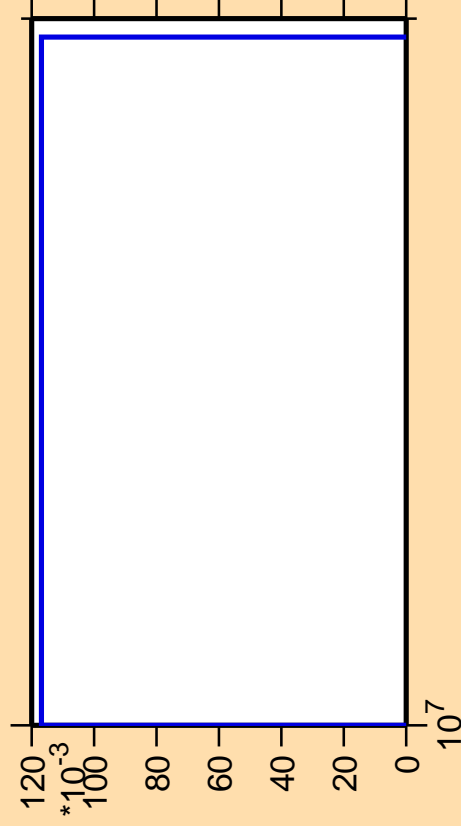
\Delta\sigma/\sigma vs. E for ^{157}\text{Tb}(\text{mt117})
