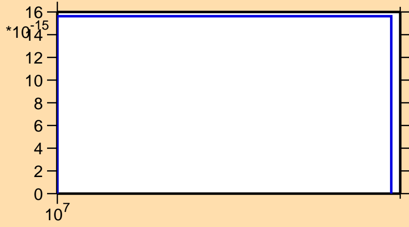
\sigma vs. E for ^{157}\text{Tb}(\text{mt117})
