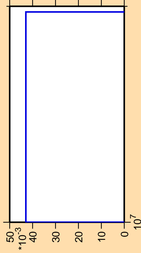
\Delta\sigma/\sigma vs. E for ^{157}\text{Tb} (mt 45)
