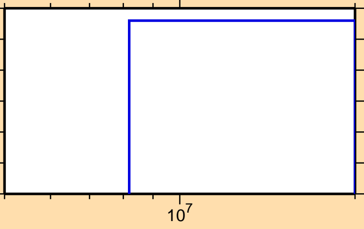
\sigma vs. E for ^{157}\text{Tb}(n,t)
