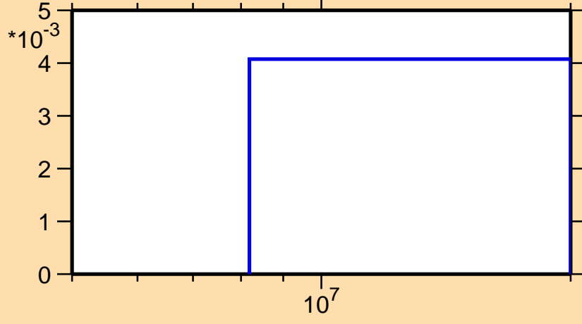
\sigma vs. E for ^{157}\text{Tb}(n,3n)
