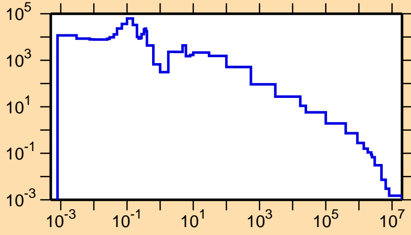
\sigma vs. E for ^{158}\text{Tb}(n,\gamma)
