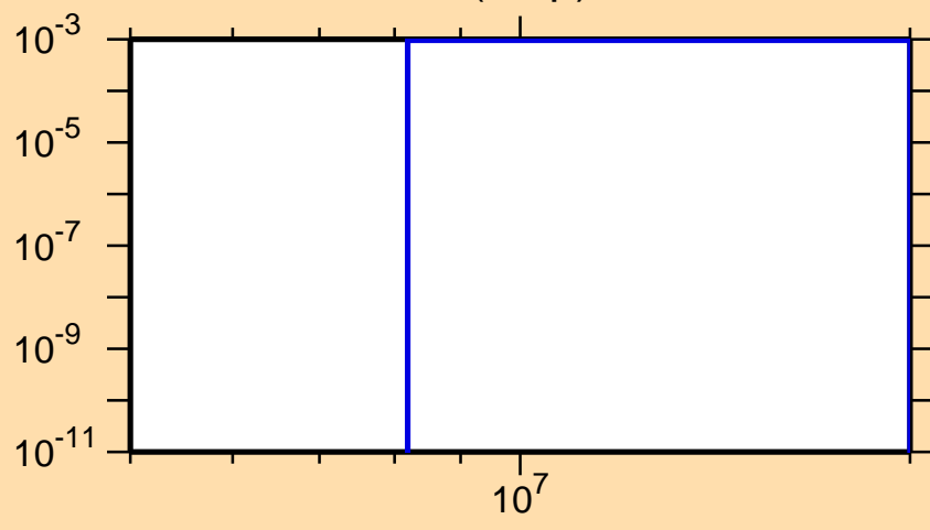
\sigma vs. E for ^{158}\text{Tb}(n,np)
