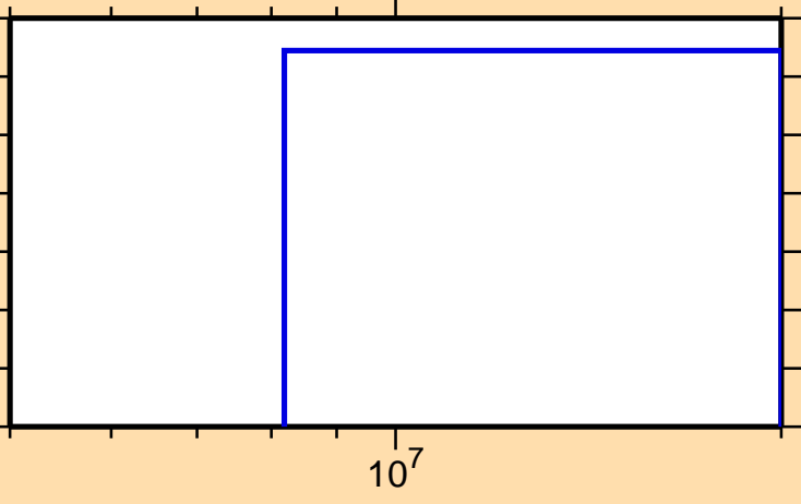
\sigma vs. E for ^{158}\text{Tb}(n,nt)
