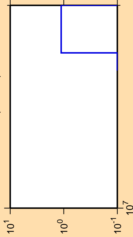
\Delta\sigma/\sigma vs. E for ^{158}\text{Tb}(\text{mt117})
