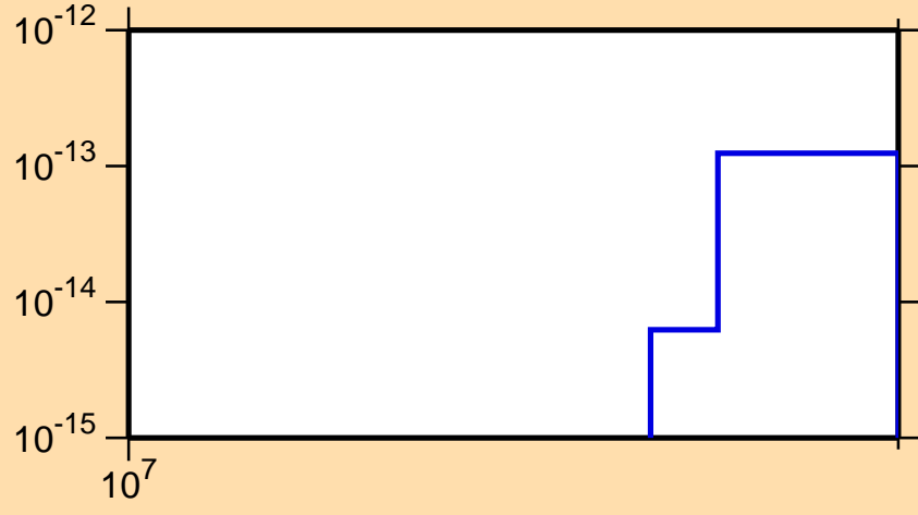
\sigma vs. E for ^{158}\text{Tb}(\text{mt117})
