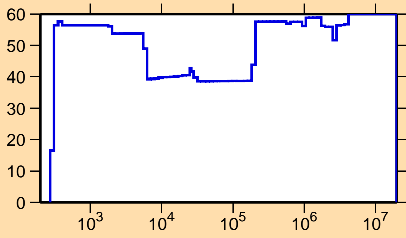
\Delta\sigma/\sigma vs. E for ^{158}\text{Tb}(n,\gamma)
