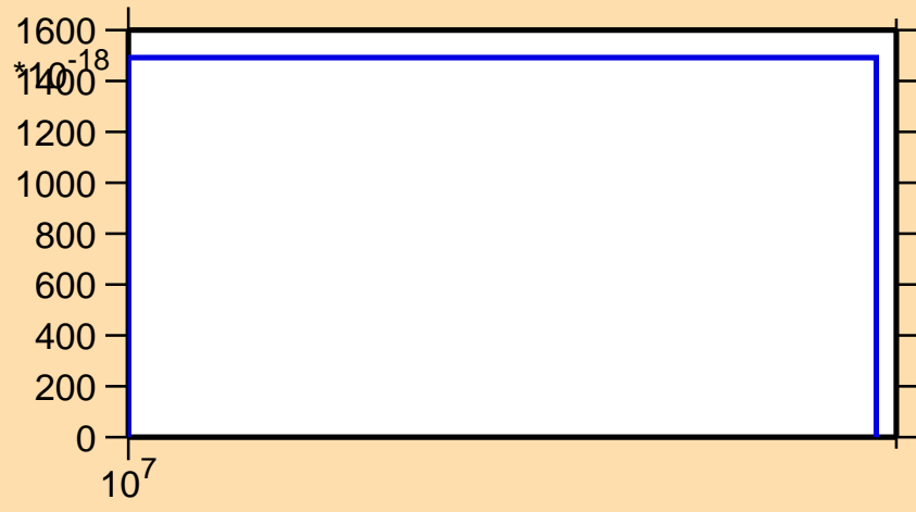
\sigma vs. E for ^{158}\text{Tb}(\text{mt117})
