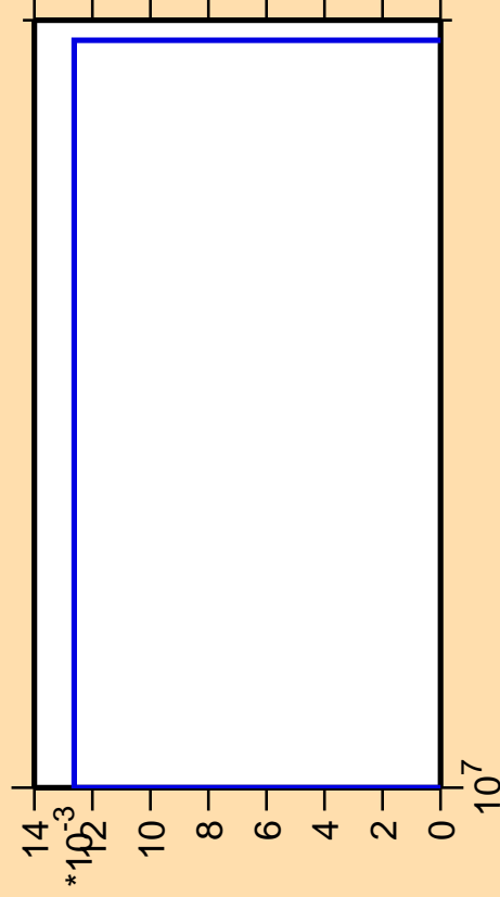
\Delta\sigma/\sigma vs. E for ^{158}\text{Tb}(\text{mt117})
