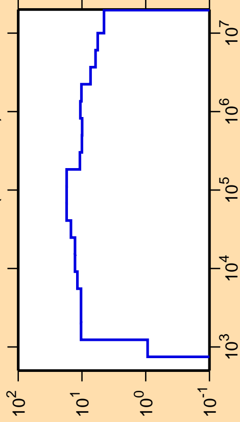
\Delta\sigma/\sigma vs. E for ^{159}\text{Tb}(n,\text{nonel.})
