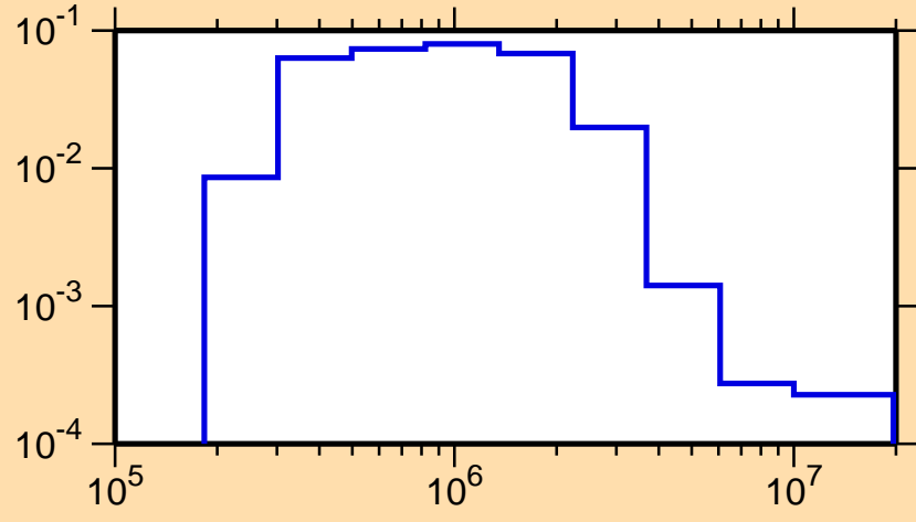
\sigma vs. E for ^{159}\text{Tb}(n,n_3)
