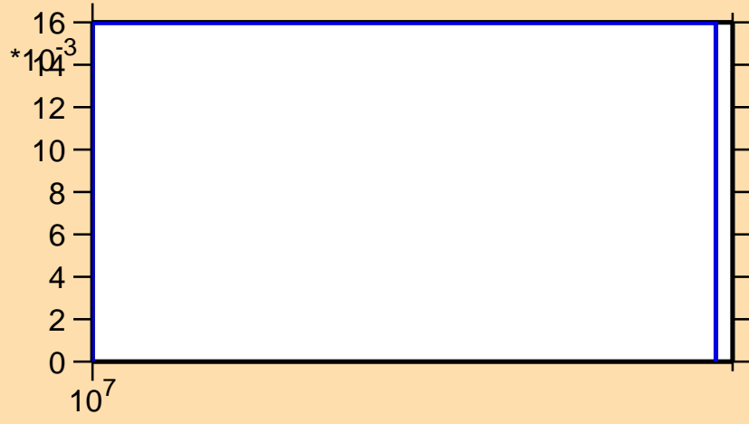
\sigma vs. E for ^{159}\text{Tb}(n,3n)
