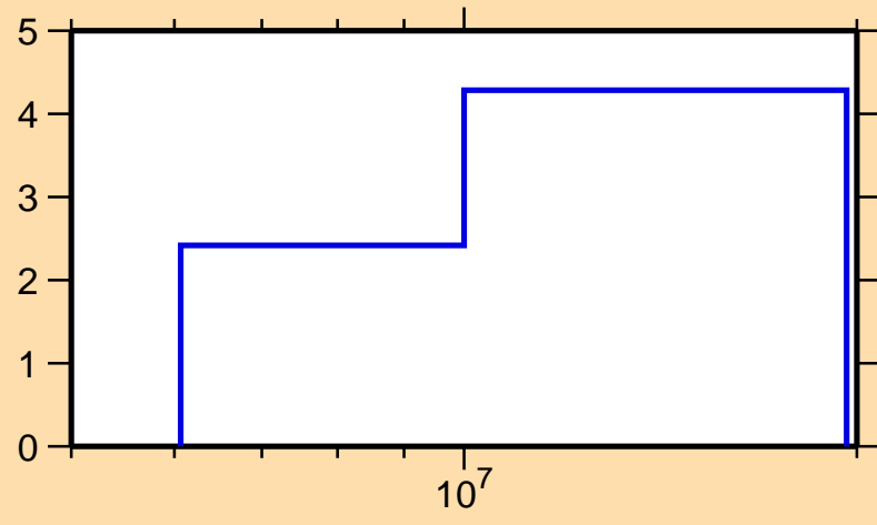
\Delta\sigma/\sigma vs. E for ^{159}\text{Tb}(n,\text{tot.})
