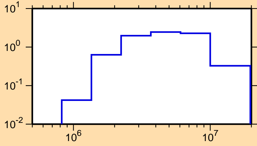
\sigma vs. E for ^{159}\text{Tb}(n,n\text{cont.})
