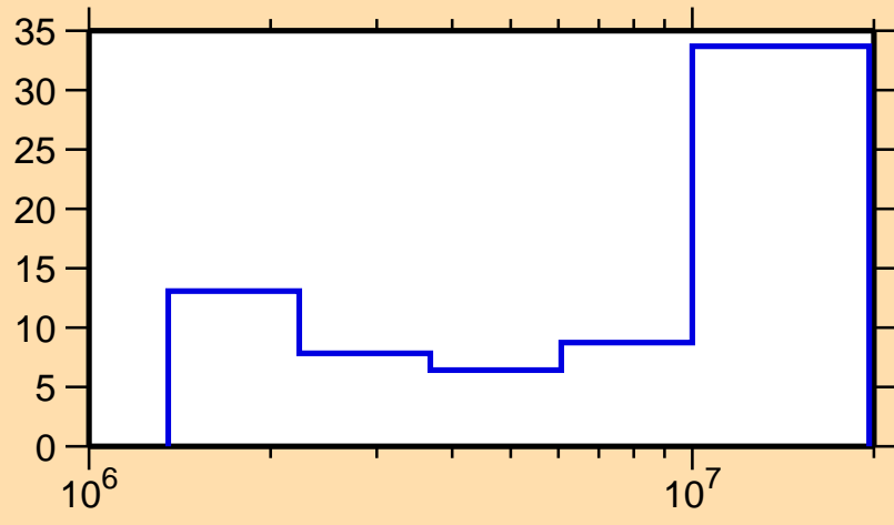
\Delta\sigma/\sigma vs. E for ^{159}\text{Tb}(n,n\text{cont.})
