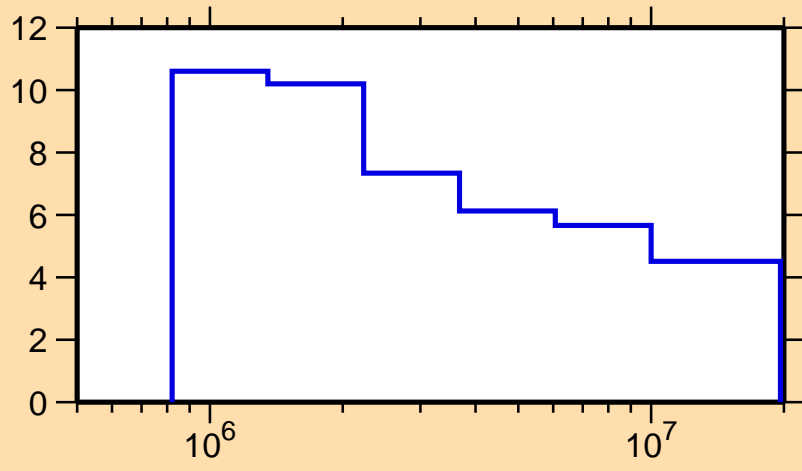
\Delta\sigma/\sigma vs. E for ^{159}\text{Tb}(n,n\text{onel.})
