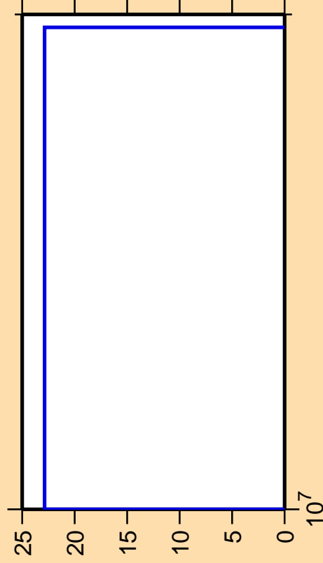
\Delta\sigma/\sigma vs. E for ^{159}\text{Tb}(n,3n)
