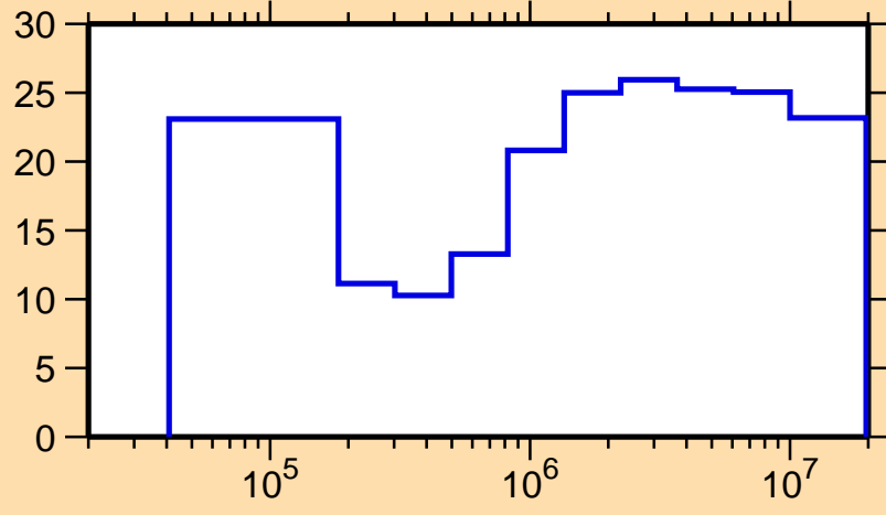
\Delta\sigma/\sigma vs. E for ^{159}\text{Tb}(n,n_1)
