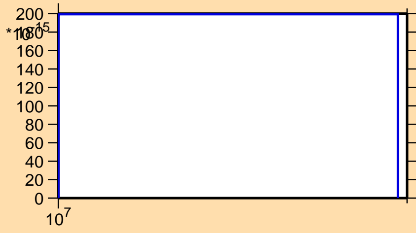
\sigma vs. E for ^{159}\text{Tb}(n,p\alpha)
