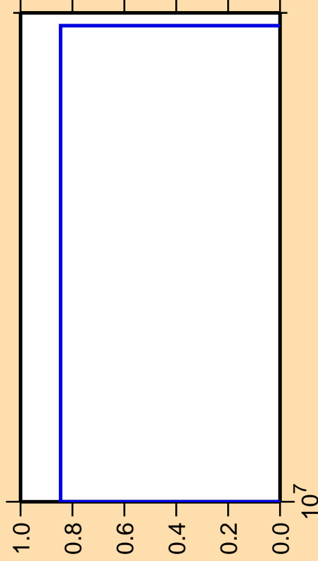
\Delta\sigma/\sigma vs. E for ^{159}\text{Tb}(n,p\alpha)
