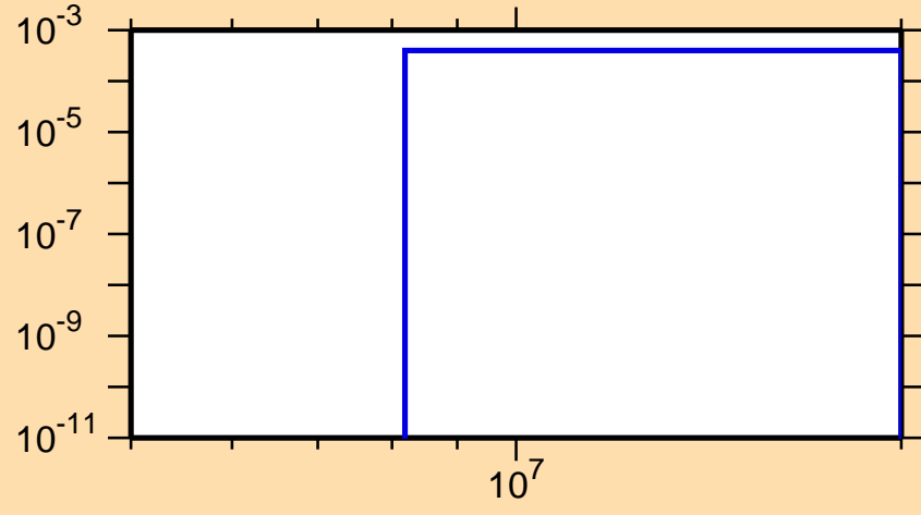
\sigma vs. E for ^{159}\text{Tb}(n,np)
