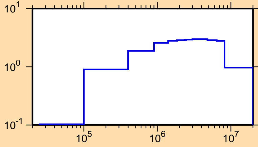
\sigma vs. E for ^{159}\text{Tb}(n,\text{inel.})
