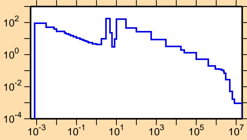
\sigma vs. E for ^{159}\text{Tb}(n,\gamma)
