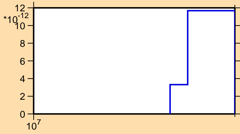
\sigma vs. E for ^{160}\text{Tb}(n,p\alpha)
