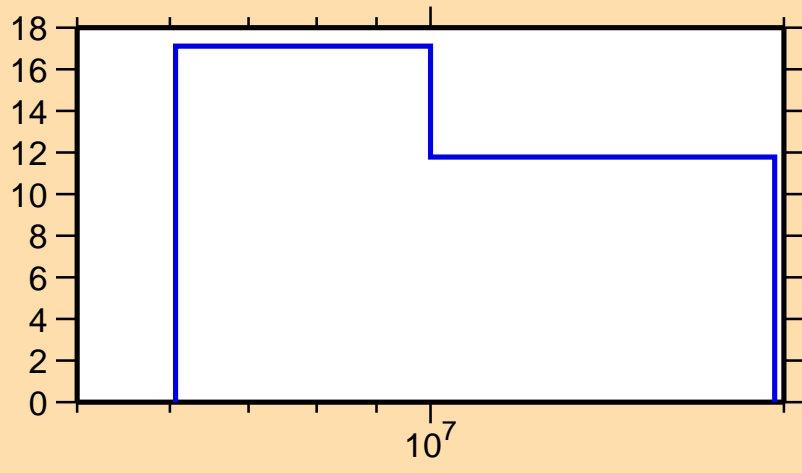
\Delta\sigma/\sigma vs. E for ^{160}\text{Tb}(n,2n)
