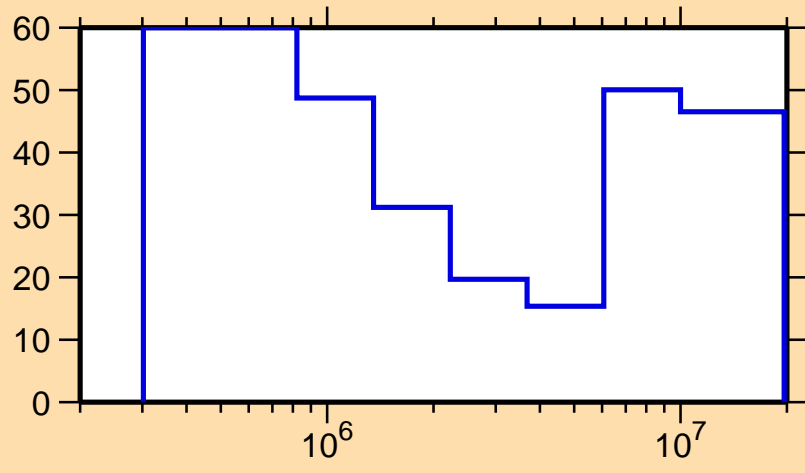
\Delta\sigma/\sigma vs. E for ^{160}\text{Tb}(n,n\text{cont.})
