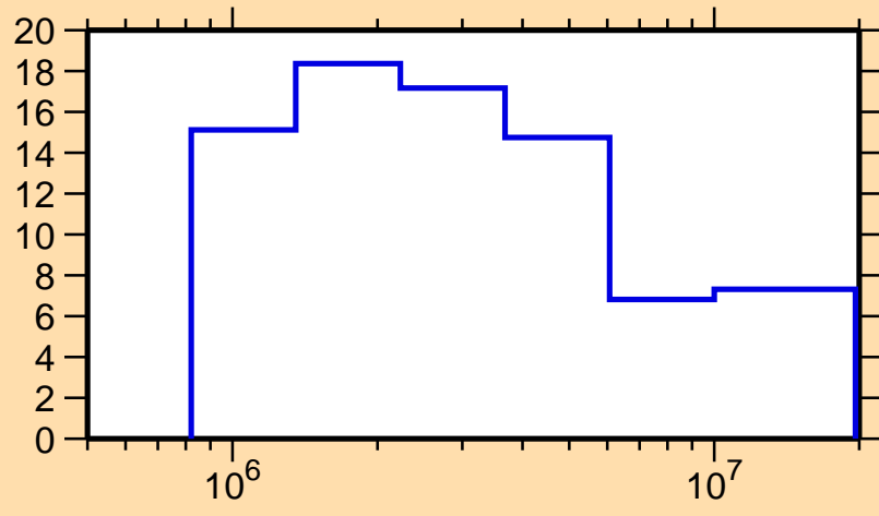
\Delta\sigma/\sigma vs. E for ^{160}\text{Tb}(n,el.)
