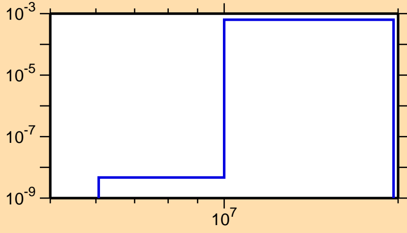
\sigma vs. E for ^{160}\text{Tb}(n,d)
