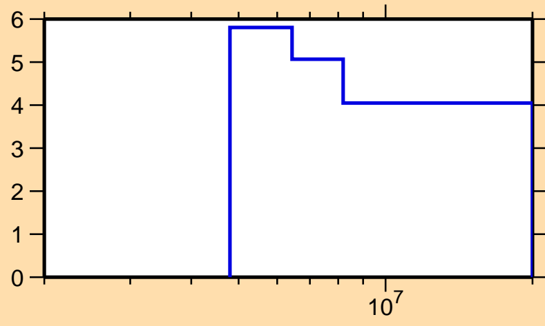
\Delta\sigma/\sigma vs. E for ^{160}\text{Tb}(n,\text{nonel.})
