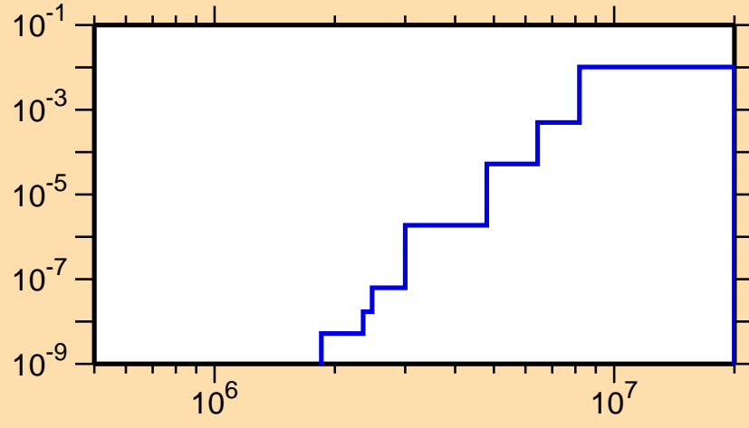
\sigma vs. E for ^{160}\text{Tb}(n,p)
