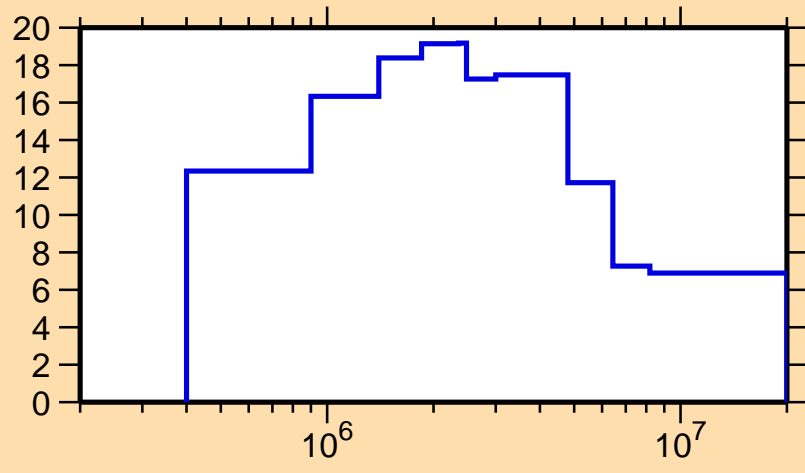
\Delta\sigma/\sigma vs. E for ^{160}\text{Tb}(n,\text{el.})
