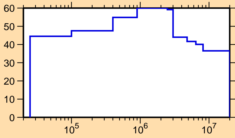
\Delta\sigma/\sigma vs. E for ^{160}\text{Tb}(n,n_1)
