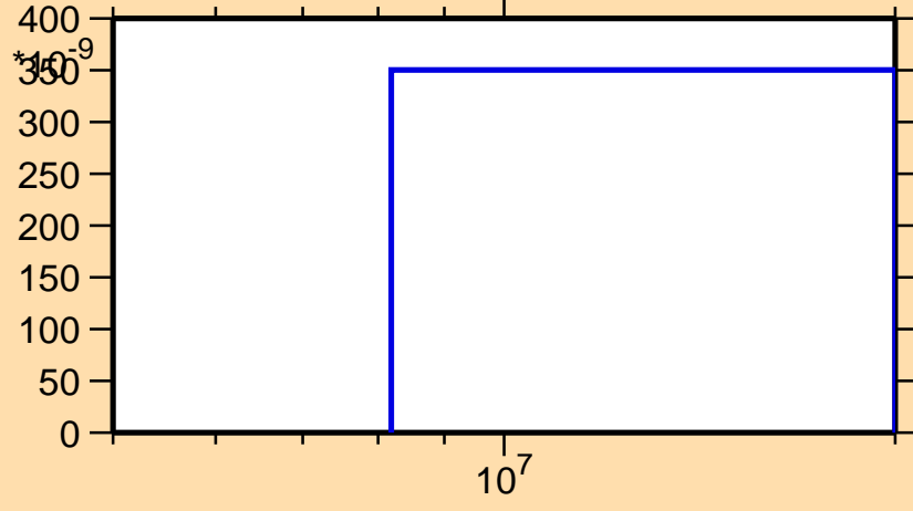
\sigma vs. E for ^{160}\text{Tb}(n,\text{nd})
