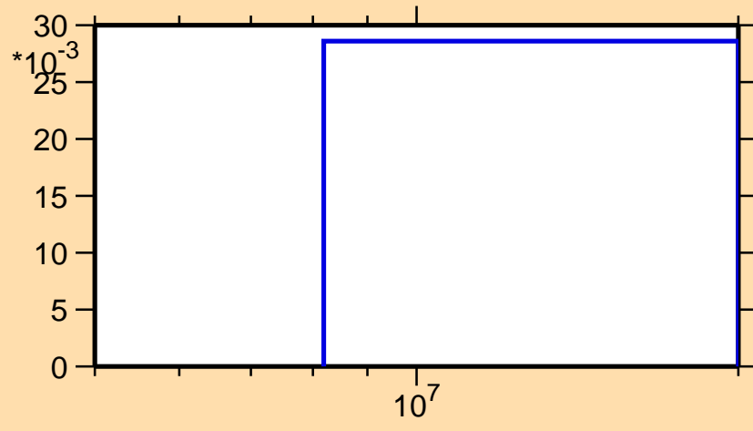
\sigma vs. E for ^{160}\text{Tb}(n,3n)
