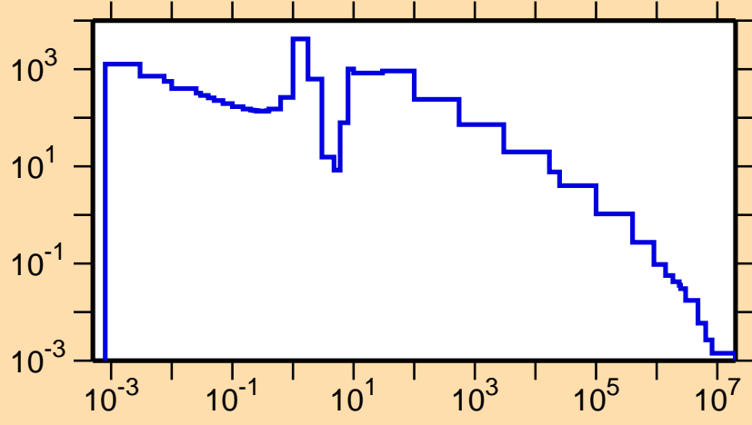
\sigma vs. E for ^{160}\text{Tb}(n,\gamma)
