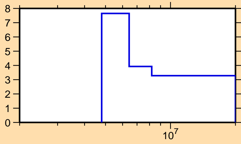
\Delta\sigma/\sigma vs. E for ^{160}\text{Tb}(n,\text{tot.})
