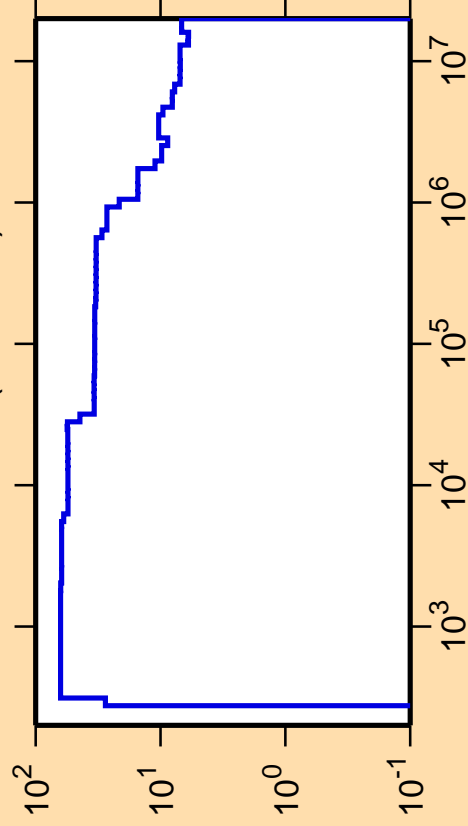
\Delta\sigma/\sigma vs. E for ^{161}\text{Tb}(n,\text{nonel.})
