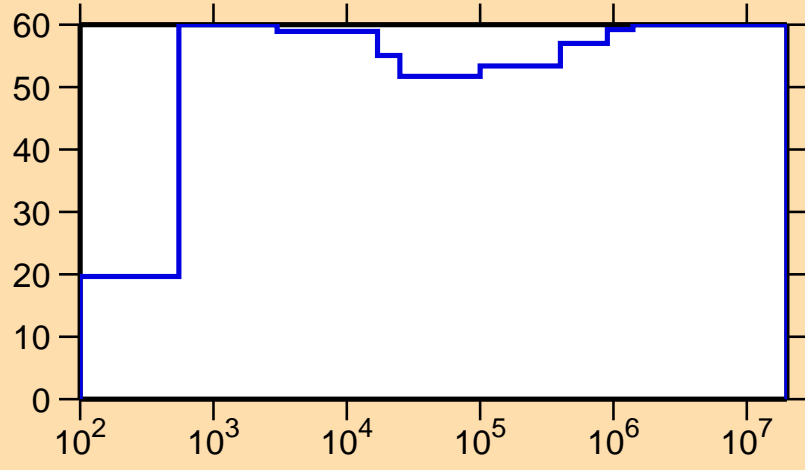
\Delta\sigma/\sigma vs. E for ^{161}\text{Tb}(n,\gamma)
