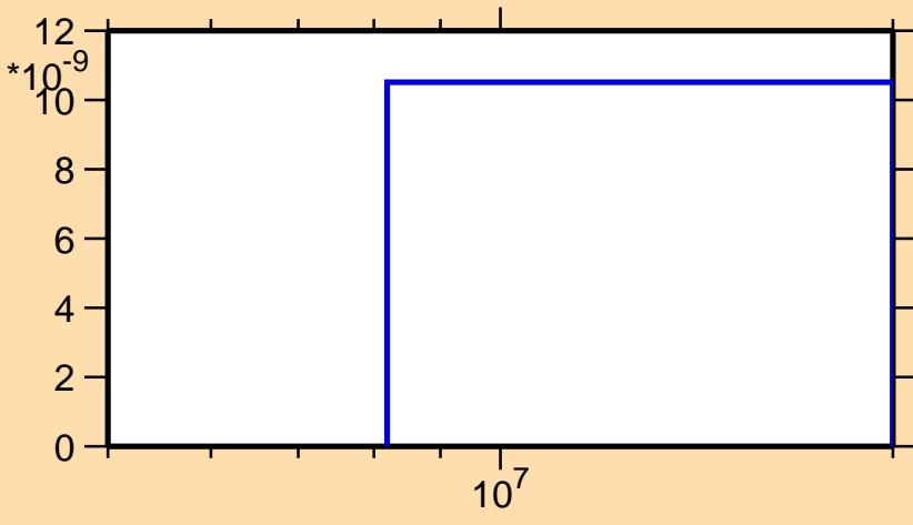
\sigma vs. E for ^{161}\text{Tb}(n,\text{nd})
