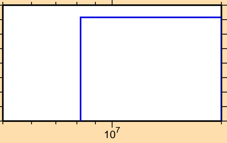
\sigma vs. E for ^{161}\text{Tb}(n,\text{He3})
