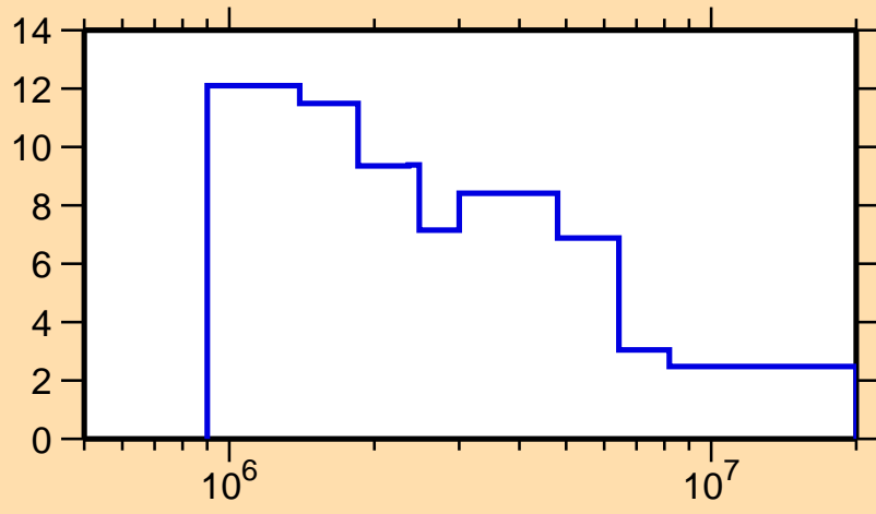
\Delta\sigma/\sigma vs. E for ^{161}\text{Tb}(n,\text{tot.})
