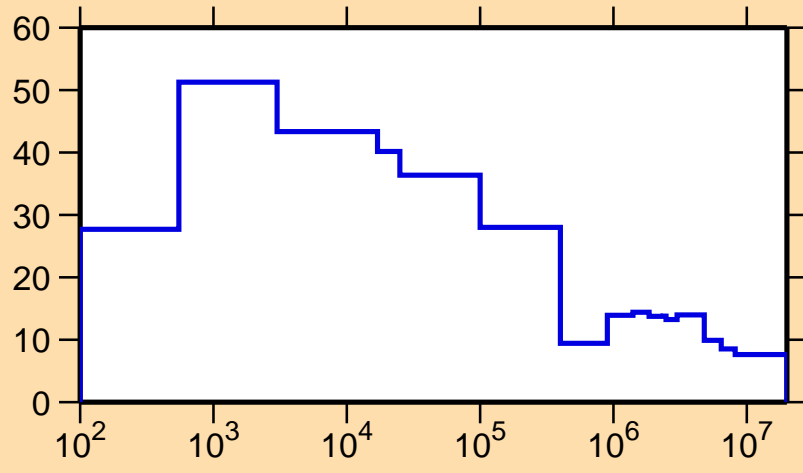
\Delta\sigma/\sigma vs. E for ^{161}\text{Tb}(n,\text{el.})
