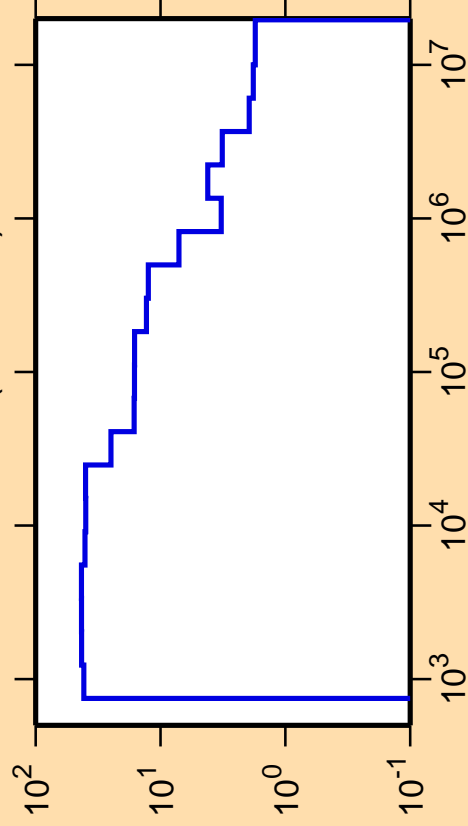
\Delta\sigma/\sigma vs. E for ^{162}\text{Tb}(n,\text{nonel.})
