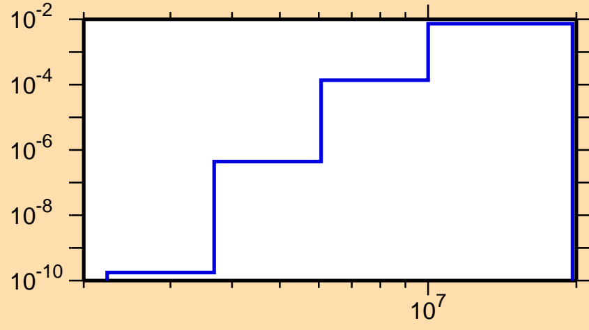
\sigma vs. E for ^{162}\text{Tb}(n,p)
