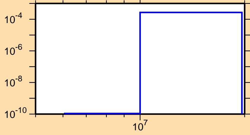
\sigma vs. E for ^{162}\text{Tb}(n,d)
