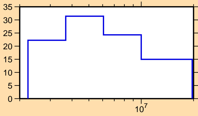
\Delta\sigma/\sigma vs. E for ^{162}\text{Tb}(n,p)
