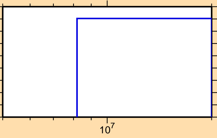
\sigma vs. E for ^{163}\text{Tb}(n,t)
