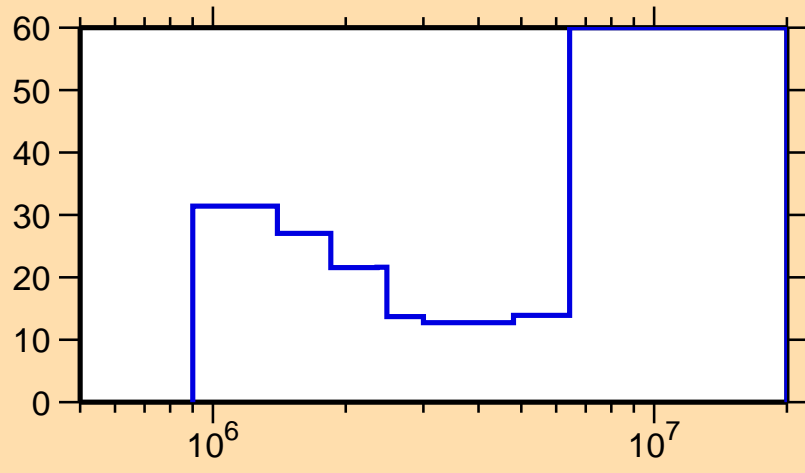
\Delta\sigma/\sigma vs. E for ^{163}\text{Tb}(n,\text{inel.})
