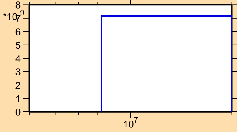
\sigma vs. E for ^{163}\text{Tb}(n,\text{nd})
