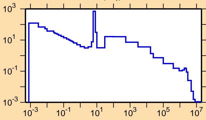
\sigma vs. E for ^{163}\text{Tb}(n,\gamma)
