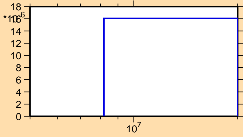
\sigma vs. E for ^{163}\text{Tb}(n,t)
