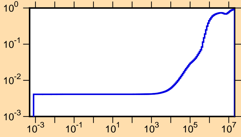
\mu vs. E for ^{164}\text{Tb}(\text{mt251})
