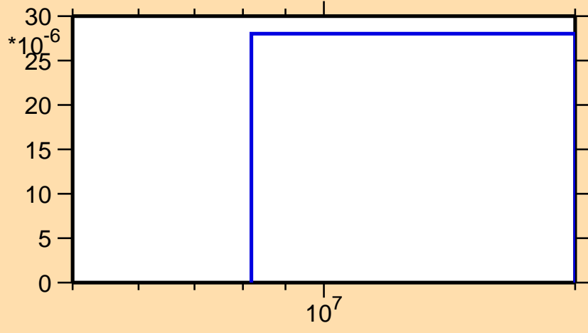
\sigma vs. E for ^{164}\text{Tb}(n,t)
