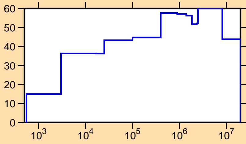
\Delta\sigma/\sigma vs. E for ^{164}\text{Tb}(n,\gamma)
