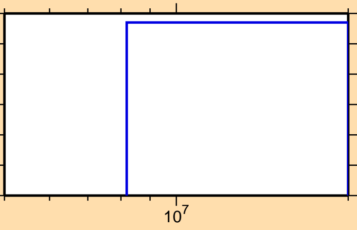
\sigma vs. E for ^{164}\text{Tb}(n,\text{nd})
