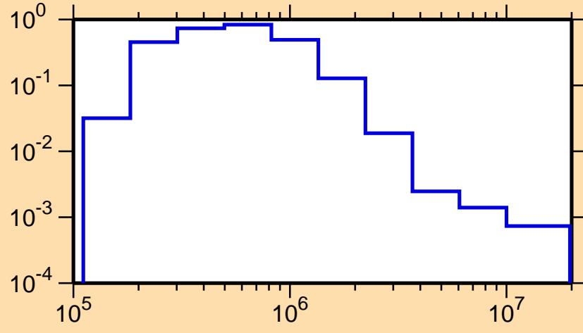
\sigma vs. E for ^{165}\text{Tb}(n,n_1)
