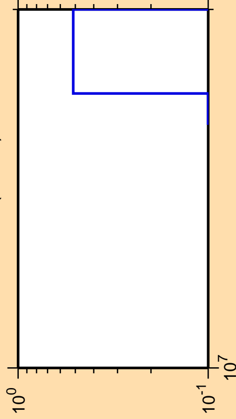
\Delta\sigma/\sigma vs. E for ^{166}\text{Tb}(n,3n\alpha)
