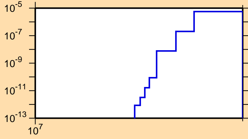
\sigma vs. E for ^{166}\text{Tb}(n,\text{nd})
