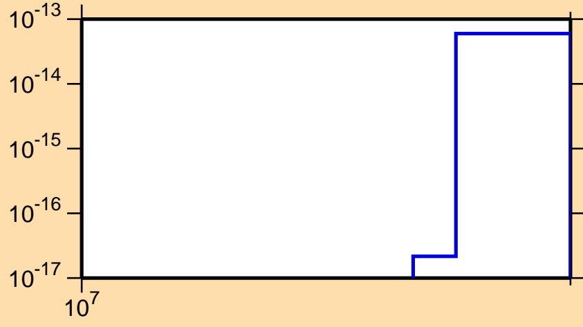
\sigma vs. E for ^{166}\text{Tb}(n,3n\alpha)
