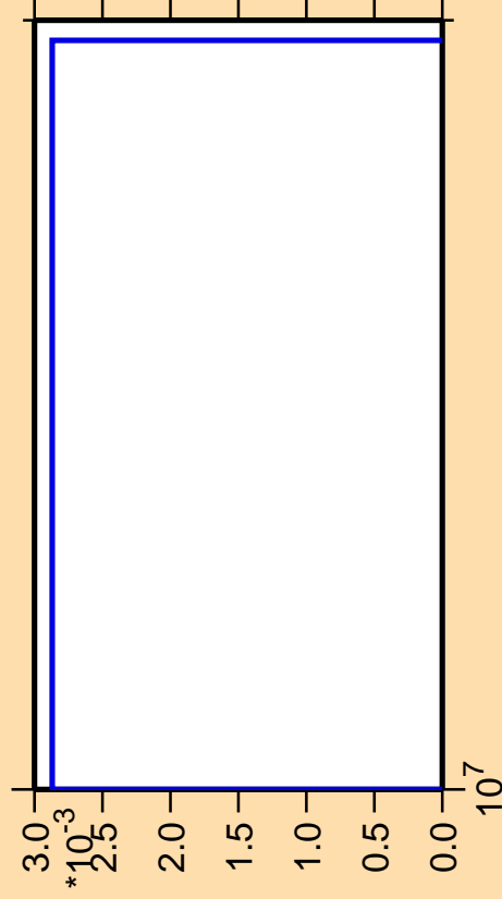
\Delta\sigma/\sigma vs. E for ^{166}\text{Tb}(n,3n\alpha)
