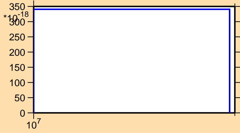
\sigma vs. E for ^{166}\text{Tb}(n,3n\alpha)
