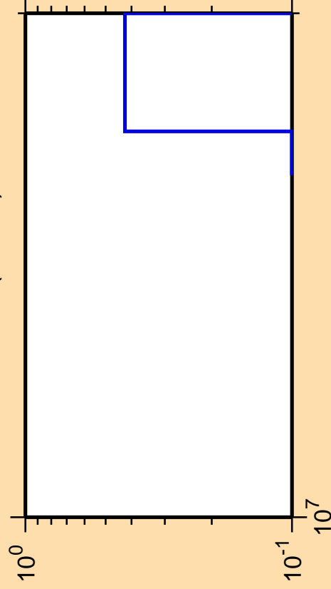
\Delta\sigma/\sigma vs. E for ^{167}\text{Tb}(n,3n\alpha)
