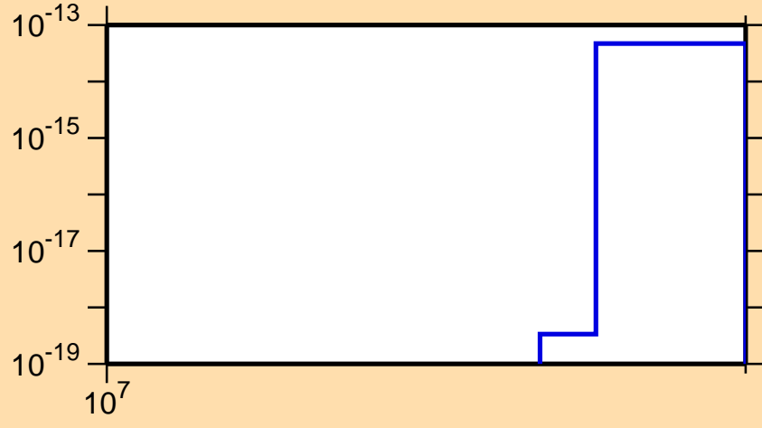
\sigma vs. E for ^{167}\text{Tb}(n,3n\alpha)
