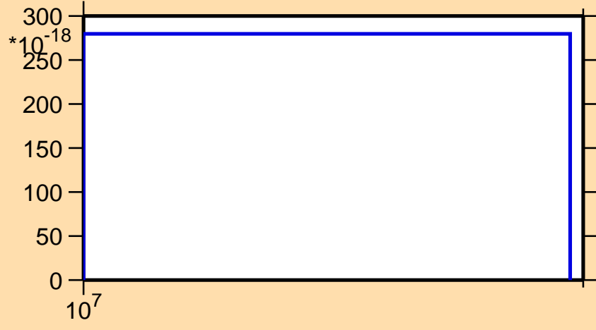
\sigma vs. E for ^{167}\text{Tb}(n,3n\alpha)
