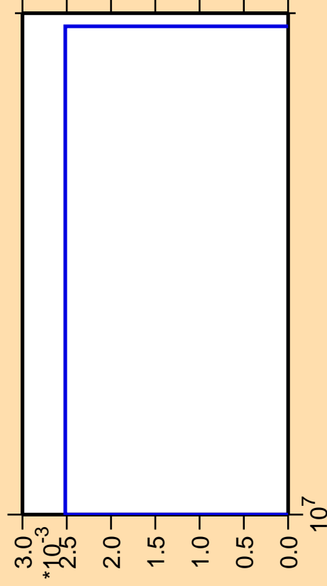
\Delta\sigma/\sigma vs. E for ^{167}\text{Tb}(n,3n\alpha)
