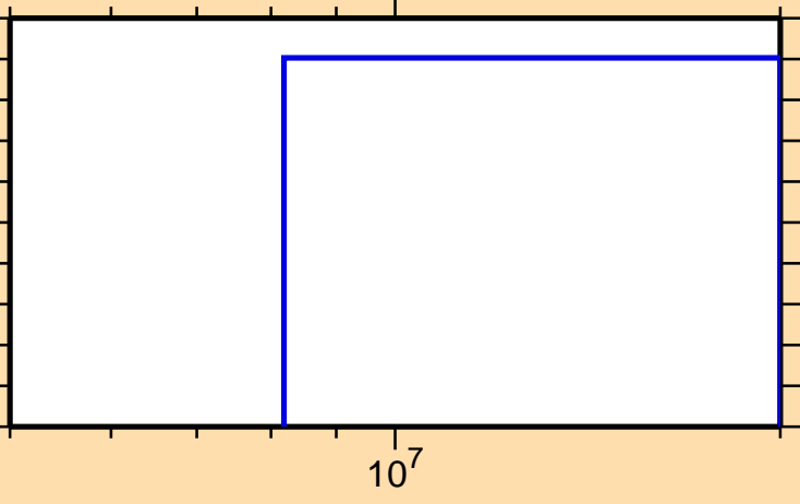
\sigma vs. E for ^{167}\text{Tb}(n,2n\alpha)
