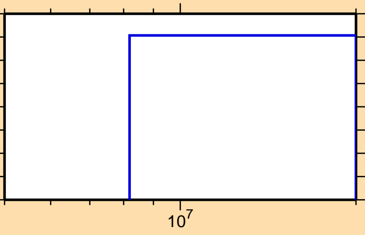
\sigma vs. E for ^{167}\text{Tb}(n,nt)
