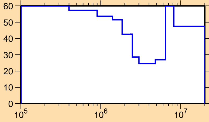
\Delta\sigma/\sigma vs. E for ^{167}\text{Tb}(n,n\text{cont.})
