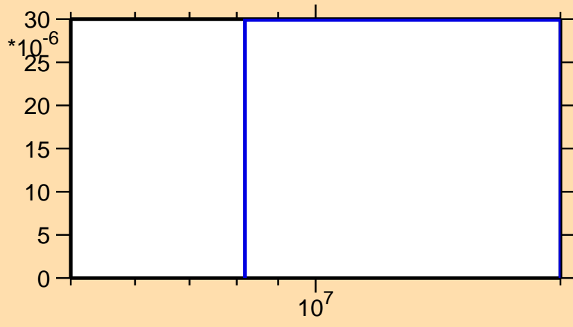
\sigma vs. E for ^{167}\text{Tb}(n,np)
