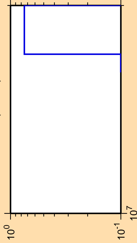
\Delta\sigma/\sigma vs. E for ^{168}\text{Tb}(n,3n\alpha)
