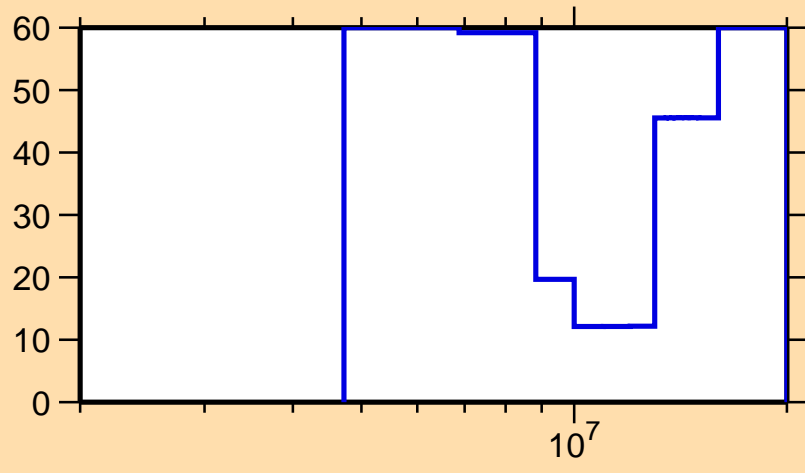
\Delta\sigma/\sigma vs. E for ^{168}\text{Tb}(n,2n)
