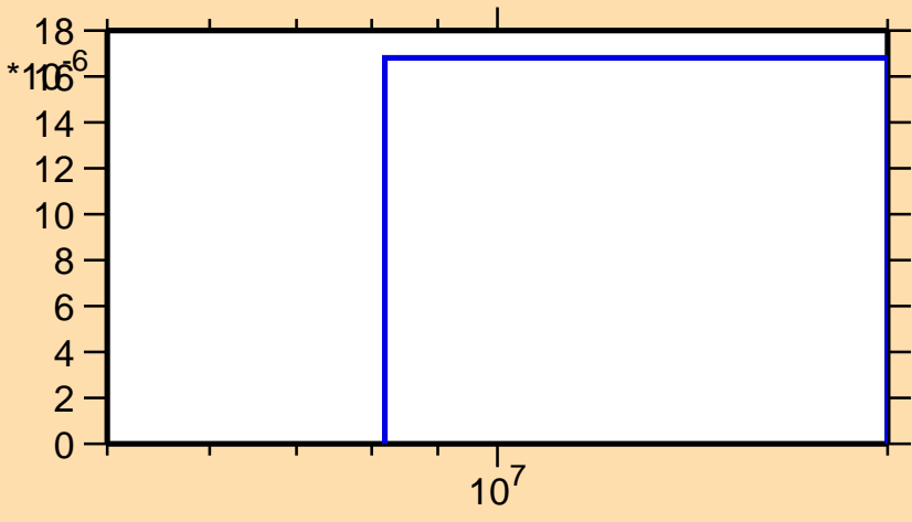
\sigma vs. E for ^{168}\text{Tb}(n,t)
