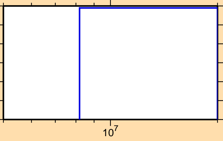
\sigma vs. E for ^{168}\text{Tb}(n,\text{nd})
