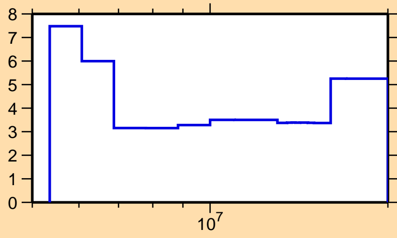
\Delta\sigma/\sigma vs. E for ^{169}\text{Tb}(n,\text{tot.})
