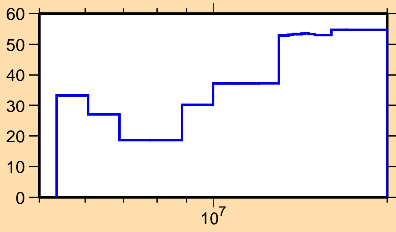
\Delta\sigma/\sigma vs. E for ^{169}\text{Tb}(n,2n)
