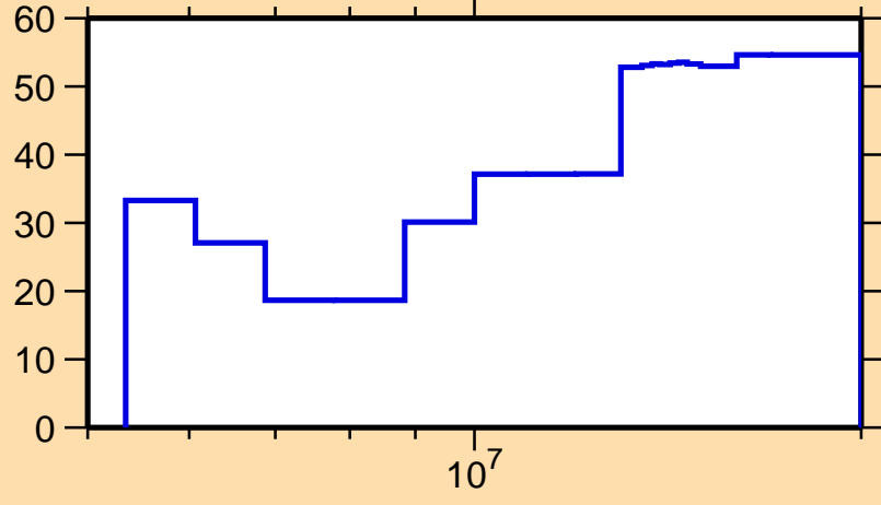
\Delta\sigma/\sigma vs. E for ^{169}\text{Tb}(n,2n)
