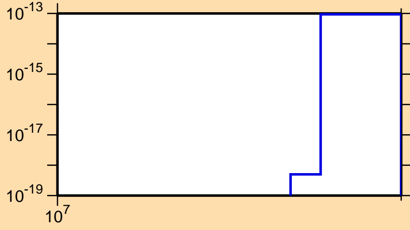
\sigma vs. E for ^{169}\text{Tb}(n,3n\alpha)
