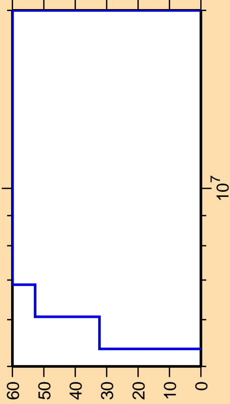
\Delta\sigma/\sigma vs. E for ^{169}\text{Tb}(n,n\text{cont.})
