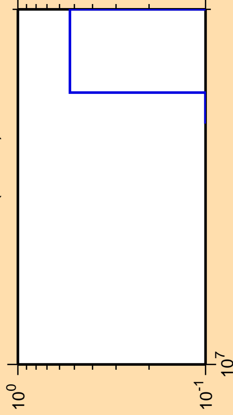
\Delta\sigma/\sigma vs. E for ^{169}\text{Tb}(n,3n\alpha)
