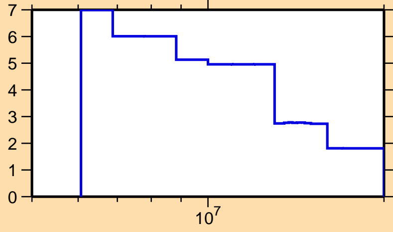
\Delta\sigma/\sigma vs. E for ^{169}\text{Tb}(n,\text{nonel.})
