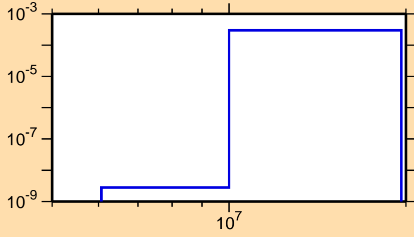
\sigma vs. E for ^{169}\text{Tb}(n,p)
