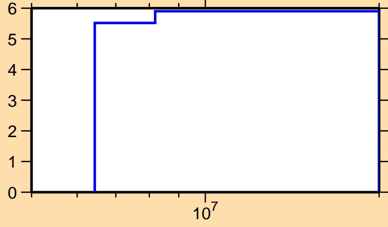
\Delta\sigma/\sigma vs. E for ^{169}\text{Tb}(n,\text{el.})
