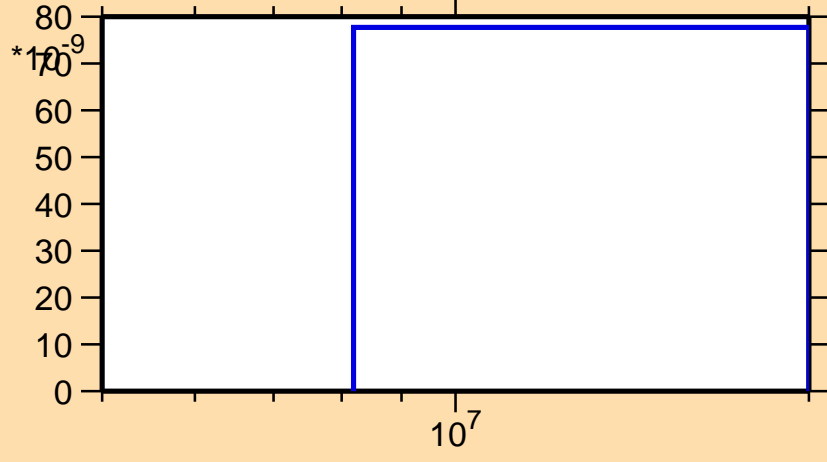
\sigma vs. E for ^{169}\text{Tb}(n,nt)
