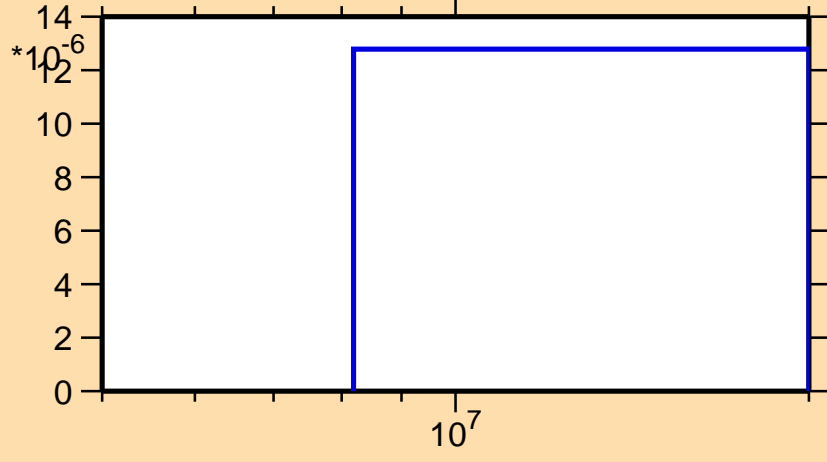
\sigma vs. E for ^{169}\text{Tb}(n,np)
