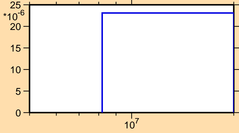
\sigma vs. E for ^{169}\text{Tb}(n,d)
