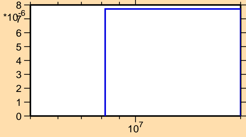
\sigma vs. E for ^{169}\text{Tb}(n,t)
