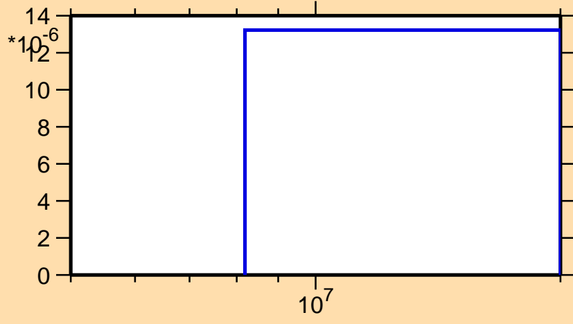
\sigma vs. E for ^{170}\text{Tb}(n,t)
