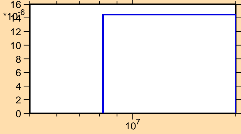
\sigma vs. E for ^{170}\text{Tb}(n,d)
