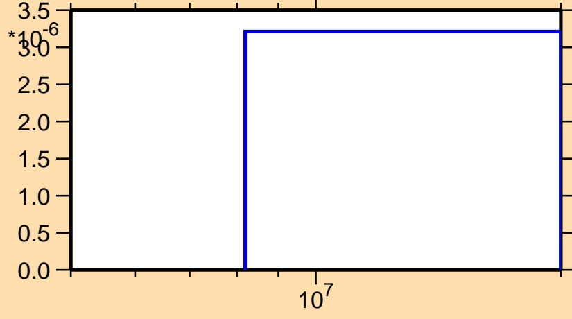
\sigma vs. E for ^{170}\text{Tb}(n,np)
