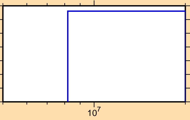
\sigma vs. E for ^{170}\text{Tb}(n,t)
