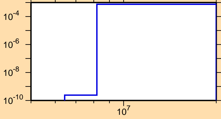
\sigma vs. E for ^{170}\text{Tb}(n,p)
