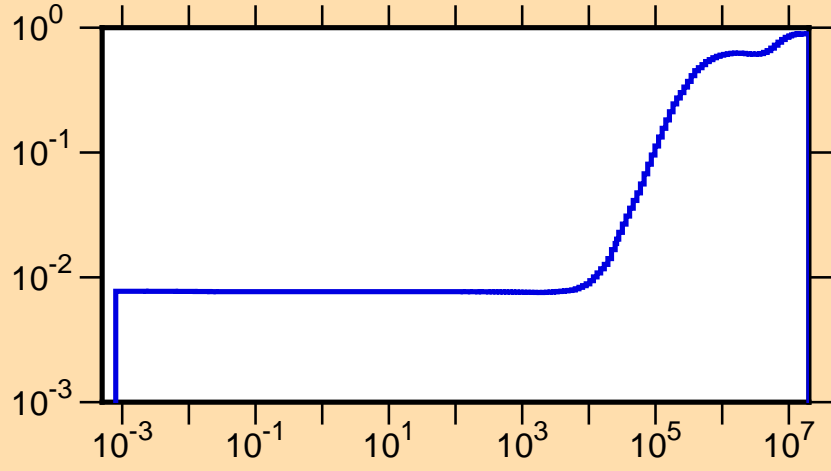
\mu vs. E for ^{87}\text{Tc}(\text{mt251})
