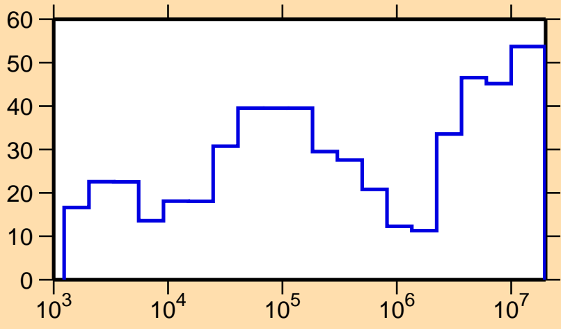
\Delta\sigma/\sigma vs. E for ^{87}\text{Tc}(n,p)
