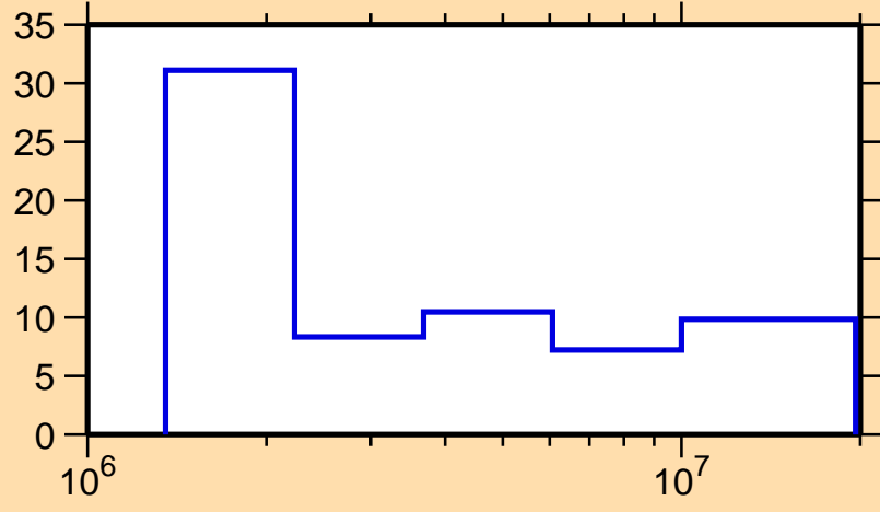
\Delta\sigma/\sigma vs. E for ^{87}\text{Tc}(n, el.)
