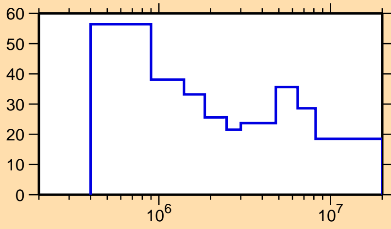
\Delta\sigma/\sigma vs. E for ^{87}\text{Tc}(n,n_1)
