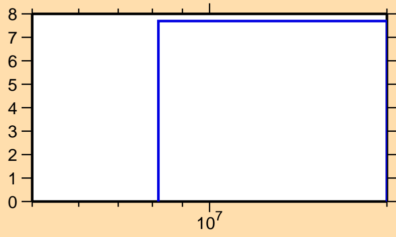
\Delta\sigma/\sigma vs. E for ^{87}\text{Tc}(n,\text{el.})
