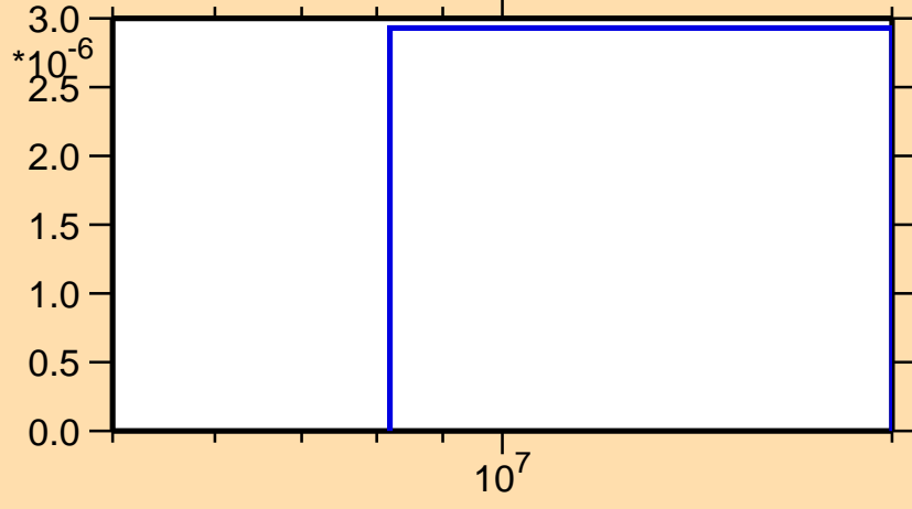
\sigma vs. E for ^{87}\text{Tc}(\text{mt } 45)
