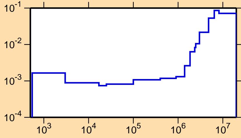
\sigma vs. E for ^{87}\text{Tc}(n,\alpha)
