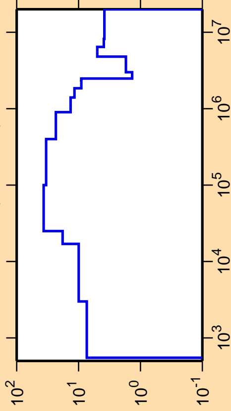
\Delta\sigma/\sigma vs. E for ^{87}\text{Tc}(n,\text{nonel.})
