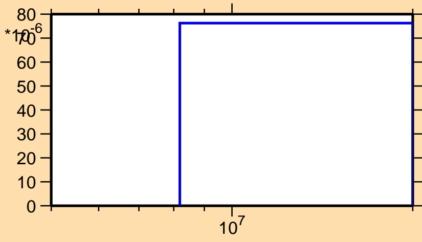
\sigma vs. E for ^{87}\text{Tc}(n,t)
