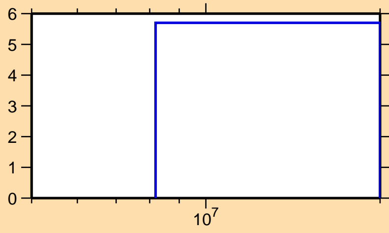
\Delta\sigma/\sigma vs. E for ^{87}\text{Tc}(n,\text{tot.})
