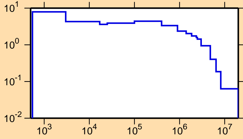
\sigma vs. E for ^{87}\text{Tc}(n,p)
