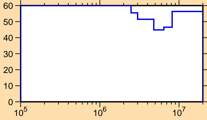
\Delta\sigma/\sigma vs. E for ^{88}\text{Tc}(n,n_1)
