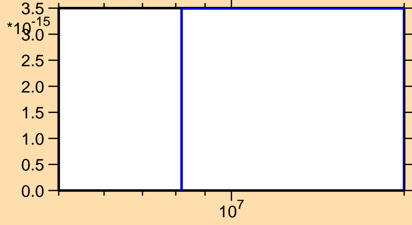
\sigma vs. E for ^{88}\text{Tc}(n,2n\alpha)
