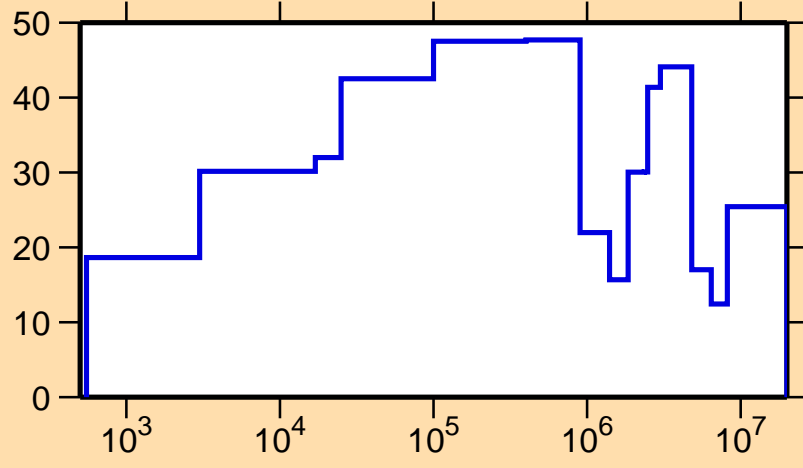
\Delta\sigma/\sigma vs. E for ^{88}\text{Tc}(n,\text{el.})
