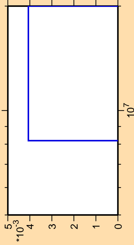
\Delta\sigma/\sigma vs. E for ^{88}\text{Tc}(n,2n\alpha)
