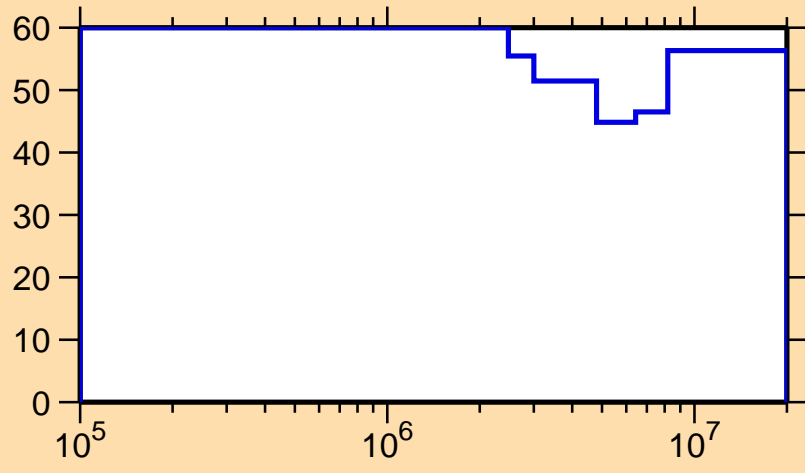
\Delta\sigma/\sigma vs. E for ^{88}\text{Tc}(n,n_1)
