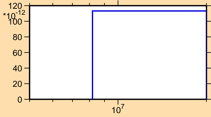
\sigma vs. E for ^{88}\text{Tc} (mt 34)
