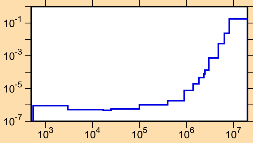
\sigma vs. E for ^{88}\text{Tc}(n,p\alpha)
