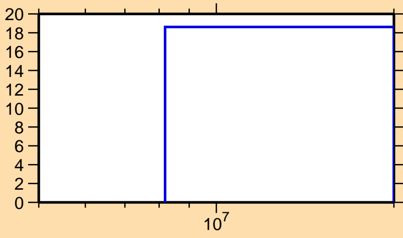
\Delta\sigma/\sigma vs. E for ^{88}\text{Tc}(n,\text{tot.})
