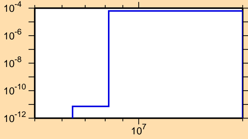
\sigma vs. E for ^{88}\text{Tc}(n,\alpha)
