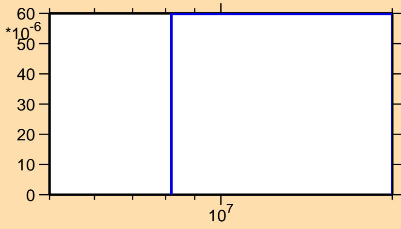
\sigma vs. E for ^{88}\text{Tc}(n,2n)
