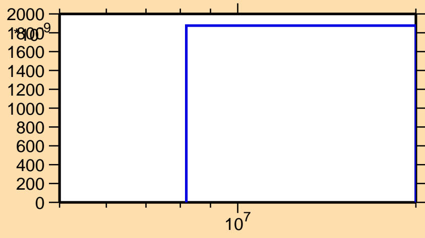
\sigma vs. E for ^{88}\text{Tc}(n,\text{pt})
