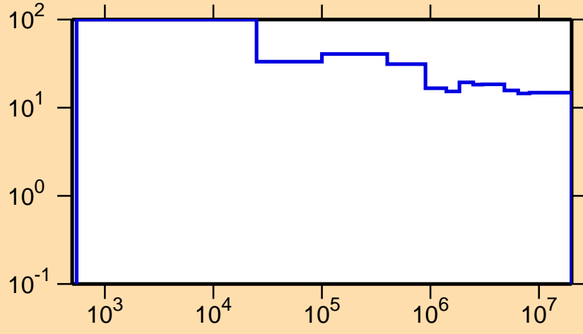
\Delta\sigma/\sigma vs. E for ^{88}\text{Tc}(n,\text{nonel.})
