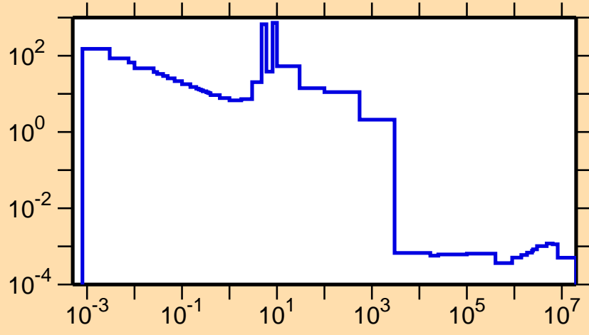
\sigma vs. E for ^{88}\text{Tc}(n,\gamma)
