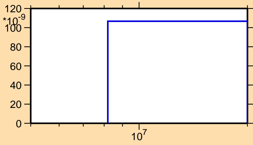
\sigma vs. E for ^{88}\text{Tc}(n,\text{nd})
