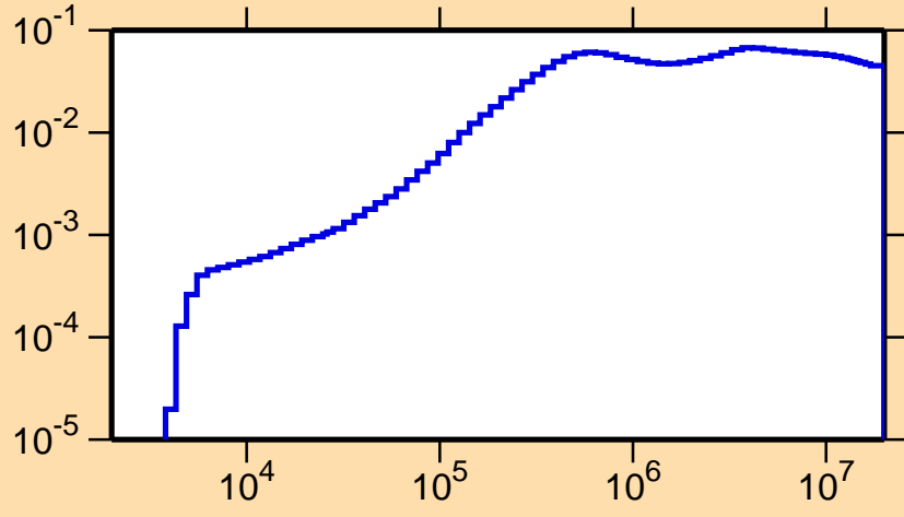
\sigma vs. E for ^{88}\text{Tc}(n,\text{inel.})
