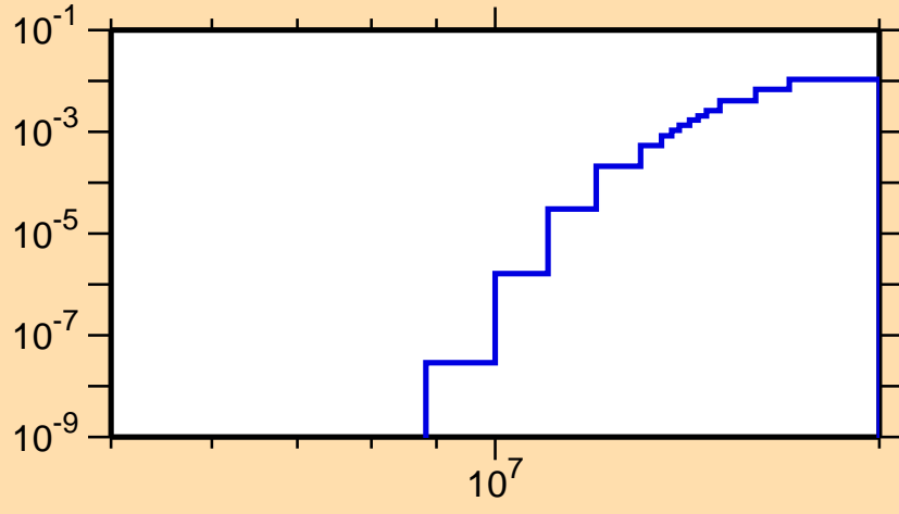
\sigma vs. E for ^{88}\text{Tc}(n,pd)
