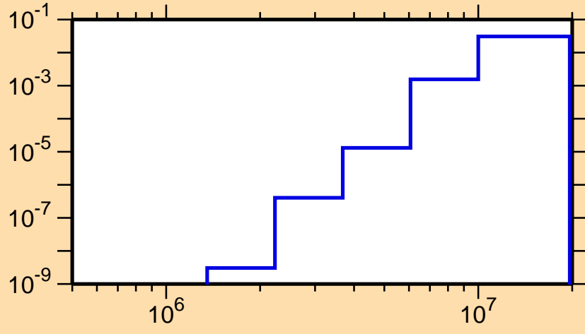
\sigma vs. E for ^{88}\text{Tc}(n,d)
