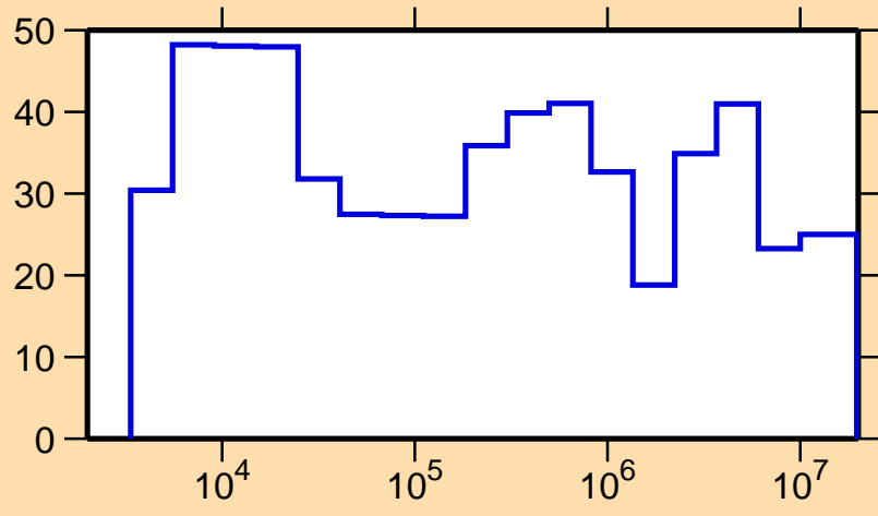
\Delta\sigma/\sigma vs. E for ^{88}\text{Tc}(n,el.)
