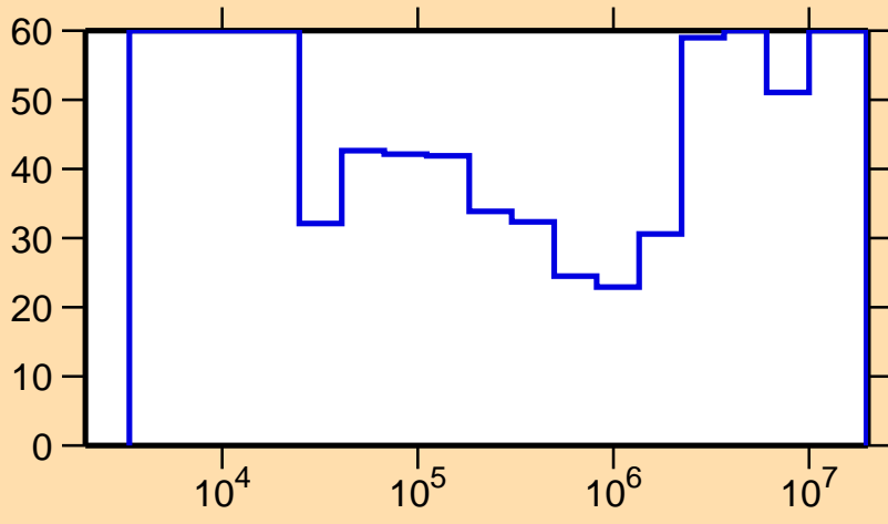
\Delta\sigma/\sigma vs. E for ^{88}\text{Tc}(n,p)
