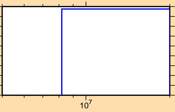
\sigma vs. E for ^{88}\text{Tc}(\text{mt117})
