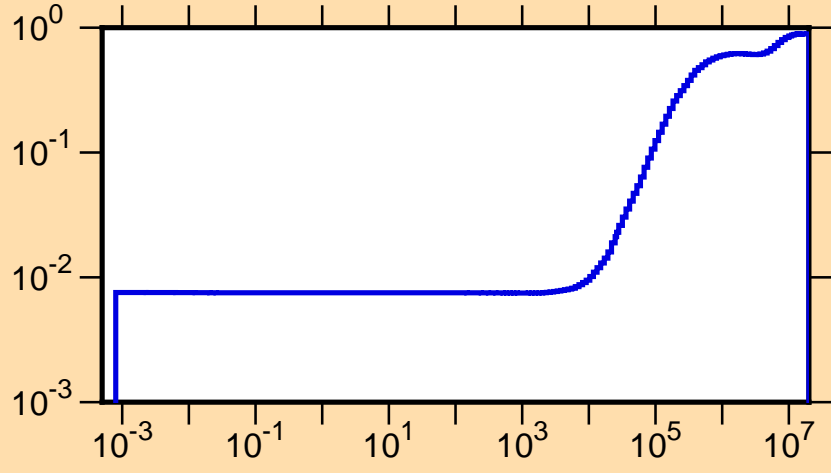
\mu vs. E for ^{89}\text{Tc}(\text{mt251})
