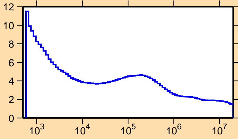
\sigma vs. E for ^{89}\text{Tc}(n,\text{nonel.})
