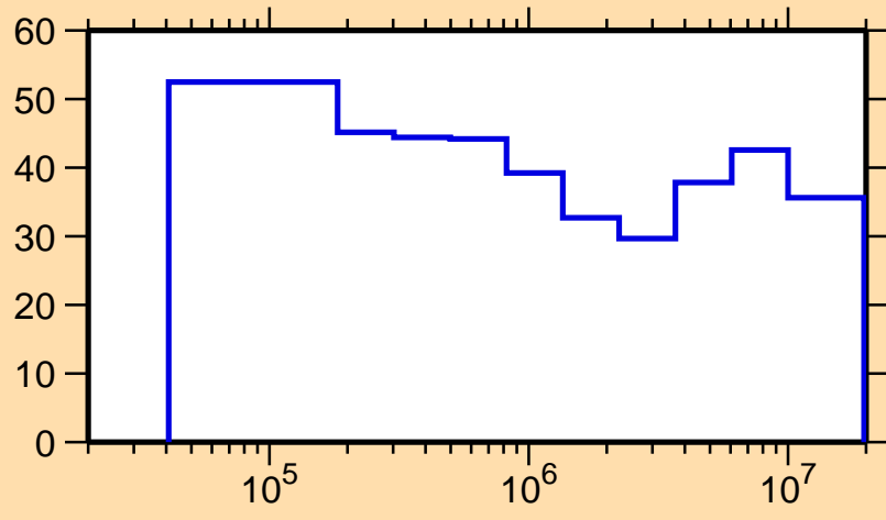
\Delta\sigma/\sigma vs. E for ^{89}\text{Tc}(n,n_1)
