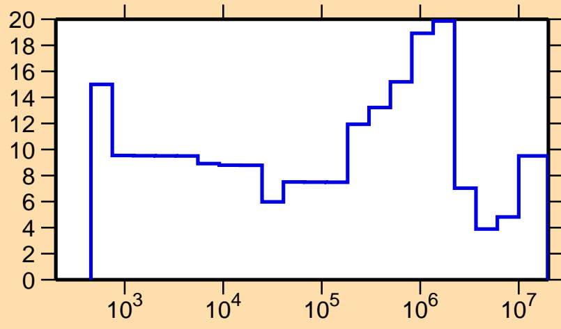
\Delta\sigma/\sigma vs. E for ^{89}\text{Tc}(n,el.)
