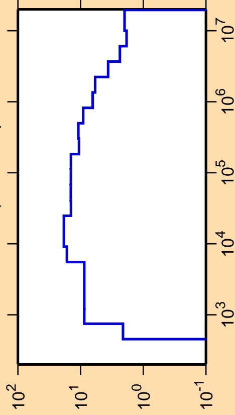
\Delta\sigma/\sigma vs. E for ^{89}\text{Tc}(n,\text{nonel.})
