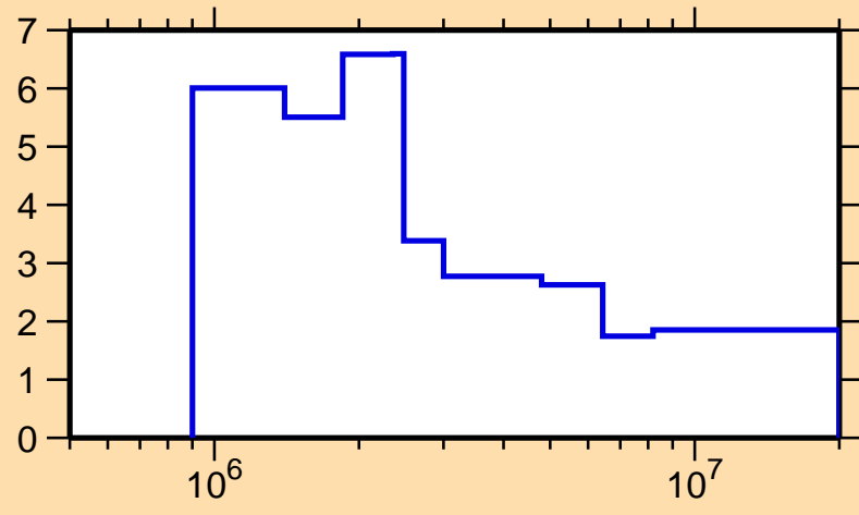
\Delta\sigma/\sigma vs. E for ^{89}\text{Tc}(n, n_{\text{nonel}})
