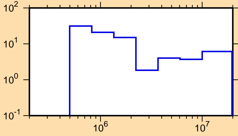
\Delta\sigma/\sigma vs. E for ^{89}\text{Tc}(n,n\text{onel.})
