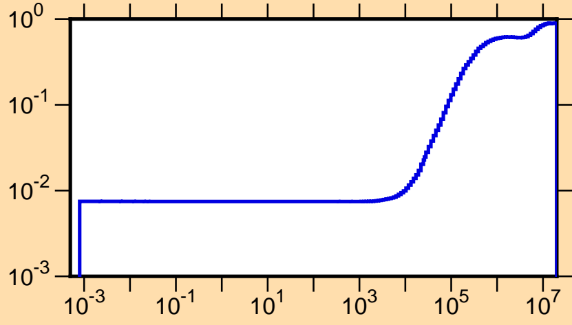
\mu vs. E for ^{90}\text{Tc}(\text{mt251})
