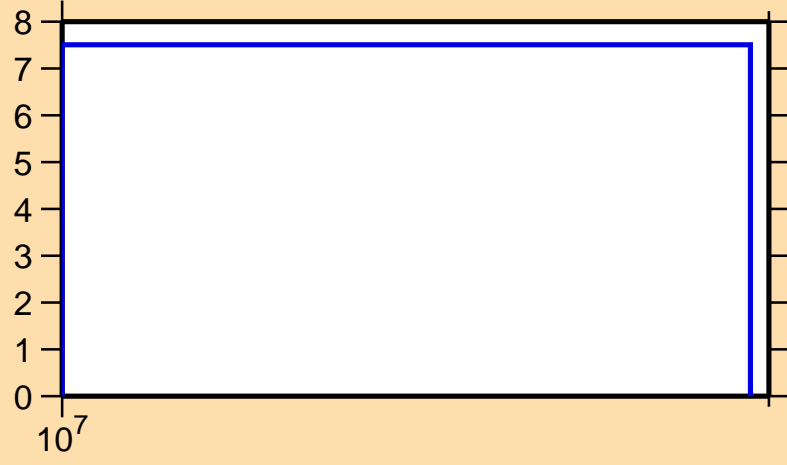
\Delta\sigma/\sigma vs. E for ^{90}\text{Tc}(n,\text{el.})
